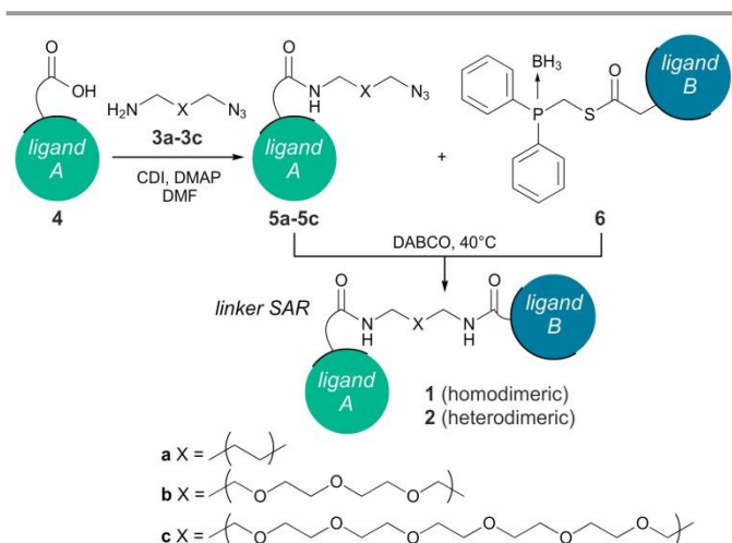
Scheme 1. The 'one-pot' PROTAC assembly approach begins with conversion of a carboxylic acid functional group 4 to its an acyl-imidazolite in situ followed by coupling to amines 3a-3c . The resulting azides 5a-5c are then coupled with thioester 6 , yielding bifunctional molecules 1a-1c and 2a-2c . We chose to use N,N -carbonyldiimidazole (CDI) for our initial study due to the ease of by-product removal, however other coupling reagents may be used.
