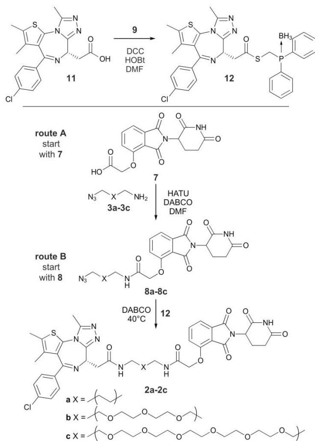
Scheme 3. Application to heterobifunctional PROTACs. Three heterodimeric PROTACs 2a-2c were assembled in a one-pot fashion beginning with 7 (route A) or 8 (route B). The choice of coupling reagent should be optimized for each system in order to consume the linker amine 3 and avoid aberrant reactivity and consumption of thioester 6 (Scheme 1). This process can be conducted on analytical scales and evaluated prior to use. One-pot procedure beginning with 7 may require HPLC purification, however starting with a collection of degrader building blocks 8 (commercially available) enables purification via standard flash column chromatography. Both methods are conducive to parallel synthesis, thereby producing all linker variants in a concerted effort from a stock solution of thioester 6 (Scheme 1).
