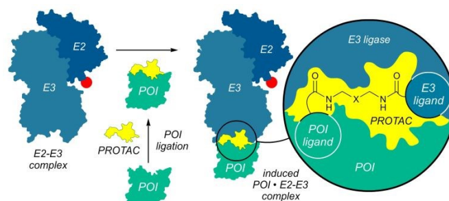
Fig. 1. Schematic representation where a heterobifunctional molecule or PROTAC (yellow) is used to target the degradation of a protein of interest (POI, green). In this process, the PROTAC contains motifs that bind to both POI and E3 ligase (blue), yielding a ternary complex. Ubiquitin (red) can then be transferred to the POI in a proximity dependent manner, leading to proteolysis of the POI.
