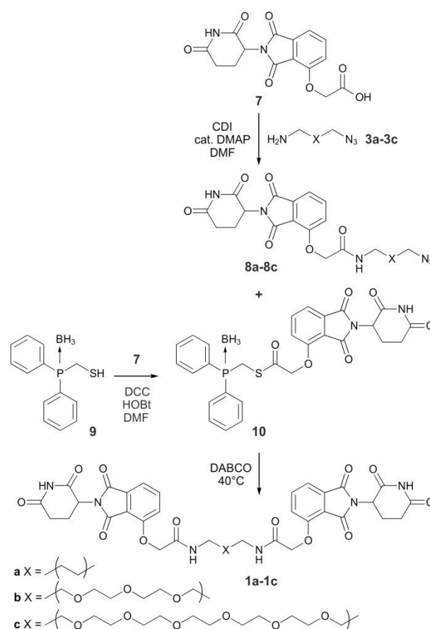
Scheme 2. Application to homobifunctional PROTACs. Three PROTACs 1a-1c were assembled in a one-pot fashion beginning with thalidomide acid 7 . Compound 10 was synthesized and isolated from thiol 9 prior to the one-pot procedure. Intermediates 8a-8c were formed in situ and were not isolated.
