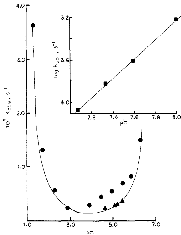
Figure 1. Hydrolysis of 3-( m -nitrophenyl)-3-methoxyphthalide; plot of k_{\text{obsd}} (●) and k_0 (▲) against pH. The calculation of the line is described in the text. The insert shows a continuation of the plot above pH 7; plot of \log k_{\text{obsd}} against pH. The buffers were HCl/KCl below pH 2.25, HOAc/NaOAc from pH 2.8–6.0, and \text{NaH}_2\text{PO}_4/\text{Na}_2\text{HPO}_4 above pH 6.2. The temperature was 70 °C. All rate constants are the average of at least two runs. \mu = 0.30 (KCl).
