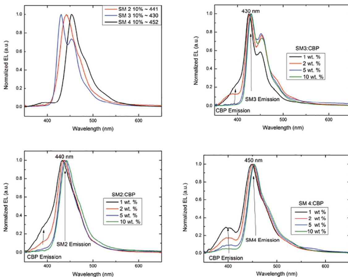
Figure 5. Electroluminescence spectra of SM2 – SM4 (top left), and EL emission at various concentrations as noted.
