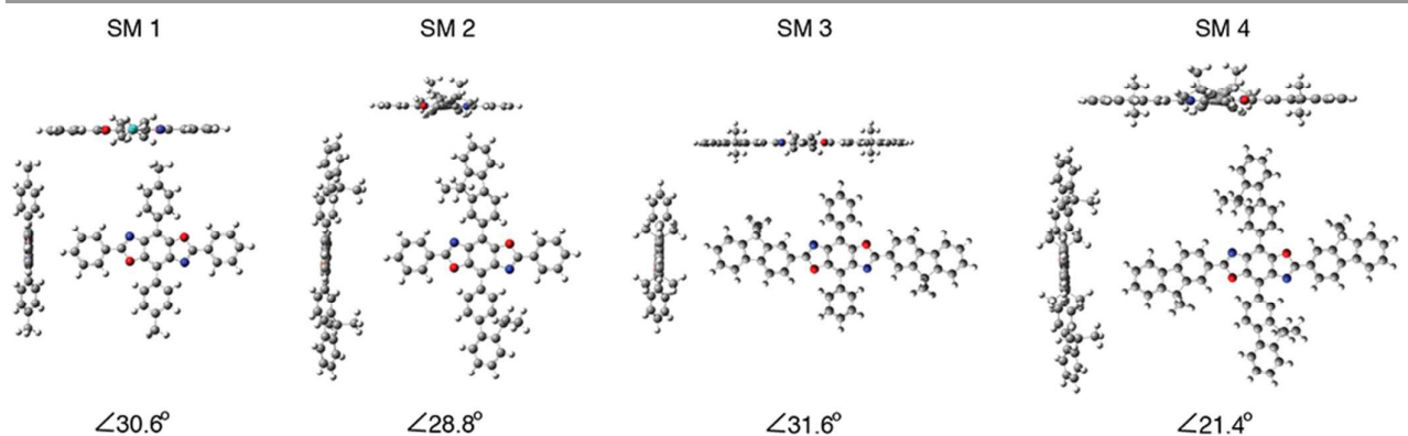
Figure 3. Optimized geometries for SM 1 – SM 4
