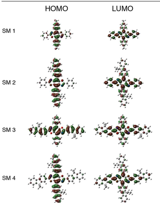
Figure 2: Frontier orbitals for SM 1 – SM 4 .
