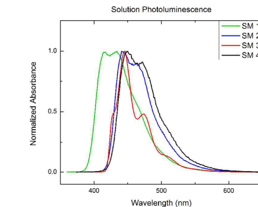
Figure 1. Photoluminescence spectra of SM 1 – SM 4 .
