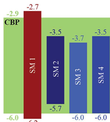
Figure 4. Energy level diagram of SM 1 – SM 4 and CBP host.
