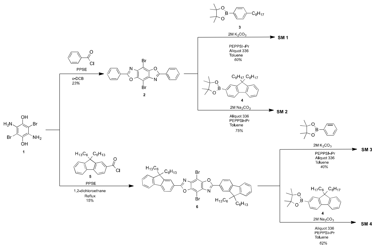
Scheme 1. Synthesis of BBO cruciform.
