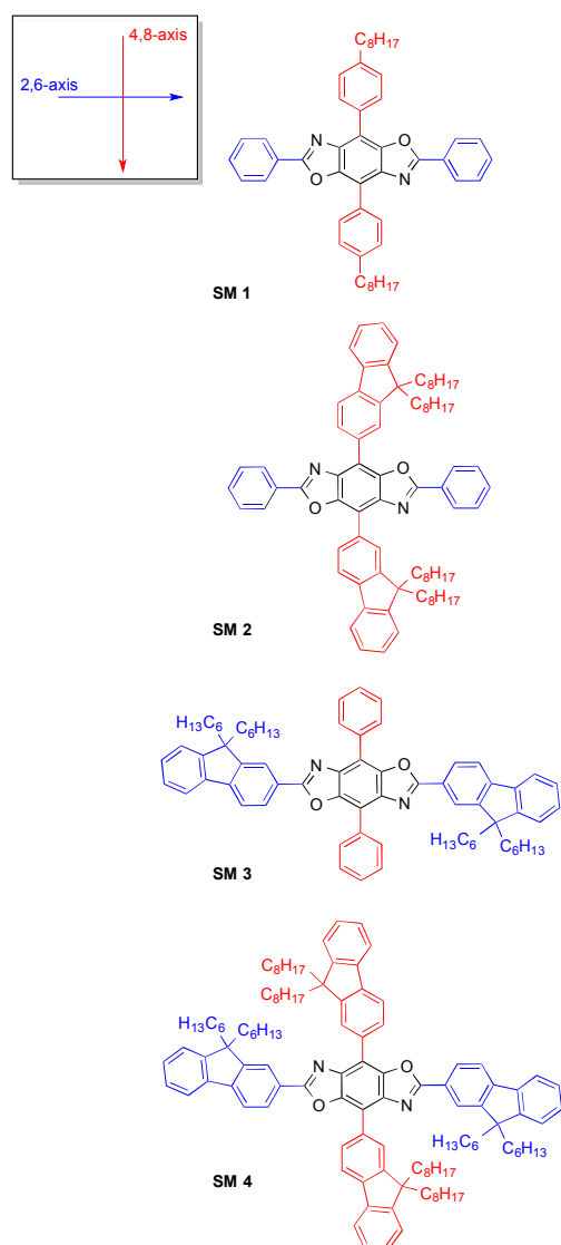
Chart 1. Structures of molecules synthesized in this work.
