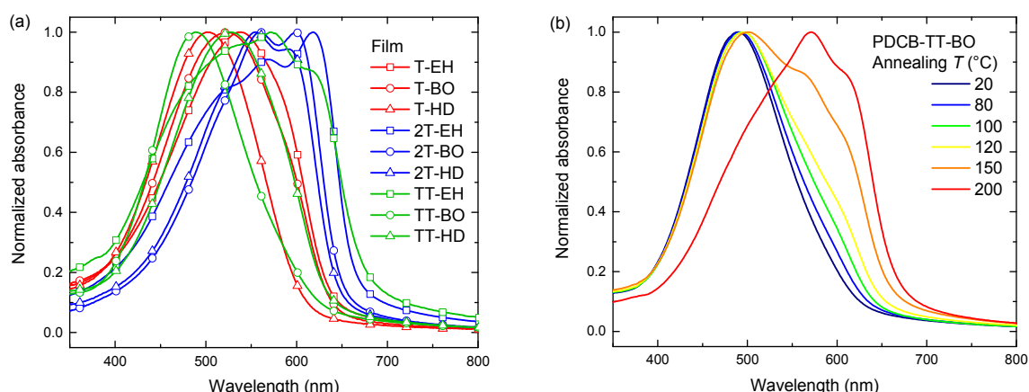
Fig. 2 (a) Optical absorption of PDCBT polymer thin films cast from chloroform. (b) Optical absorption spectra after thermal annealing of a PDCB-TT-BO film. The annealing temperature is shown in the legend, all spectra were recorded at room temperature after thermal annealing.
