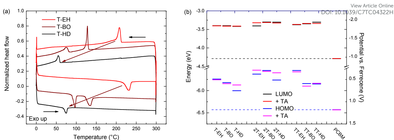
Fig. 3 (a) DSC traces of PDCB-T polymers. (b) Redox potentials and electrochemical energy levels for the PDCB polymers.
