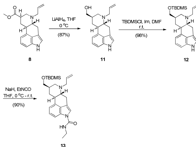
Scheme 5 Synthesis of 13 -Introduction of an ethylcarbamoyl fragment onto the indole nitrogen of lysergol derivative 12 .
