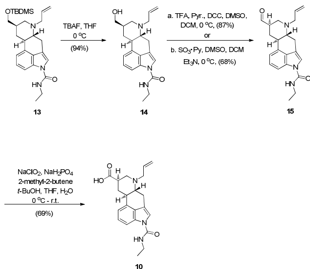
Scheme 7 Indirect, oxidative route to the 9,10-dihydrolysergal acid 10 .
