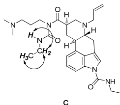
Fig. 2 Detected COSY interactions in ethylamido side chain ( CH_3 , 1.18 ppm; CH_2 , 3.30 ppm; NH , 9.45 ppm) in impurity C are indicated by arrows.
