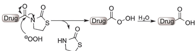
Fig. 1 Proposed scheme for activation of a thiazolidinone prodrug.
