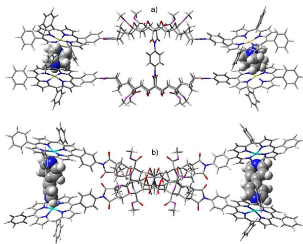
Figure 14. Molecular modelling of the zinc(II) metallated adduct of the two binding site tetra-porphyrin tweezer 2 in the presence of diamino ligands; a) 2 :(DABCO) 2 (side-on), (b) 2 :(bipy) 2 (top-down) (semi-empirical, AM1).
