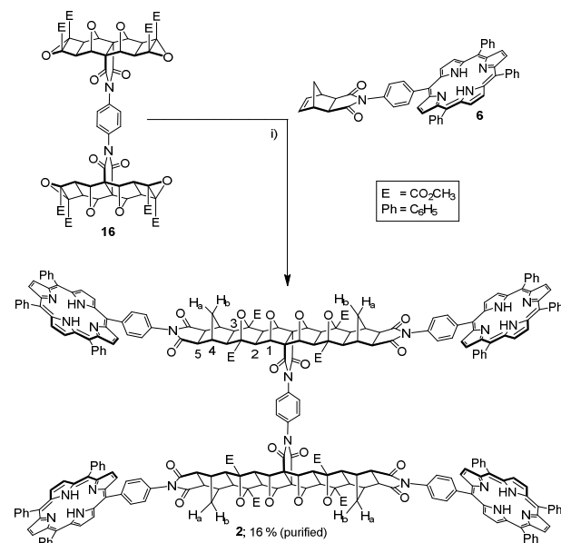
Figure 11. i) exo -porphyrin receptor 6 (4 eq.), dry THF, microwave 80-220 W, 14-20 bar, 170 °C, 2 hrs, 16 % after purification.
