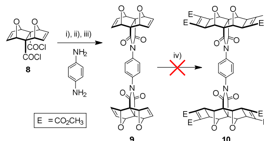
Figure 5. i) p -phenylenediamine, THF, N 2 atmosphere, r.t., slow addition of <1 eq. LiHMDS, stirring 30 mins, ii) diacid chloride (2 eq.), N 2 atmosphere, r.t., 1 hr, iii) HOBT/DCC/Et 3 N, dry THF, N 2 atmosphere, r.t., 3 days; iv) DMAD (4 eq.), 20 mol-% [Ru(H 2 CO(PPh 3 ) 3 )], dry DMF, 60 °C, N 2 atmosphere, 24 hrs, no reaction.
