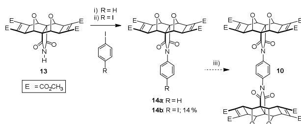
Figure 9. i) 1-iodobenzene (excess, as solvent), freshly precipitated Cu(0) (5 eq.), 4x 10 minute microwave cycles (300 W, high stirring, air cooling, 150 °C); ii) Initially 1,4-diiodobenzene (8 eq.), freshly precipitated Cu(0) (8 eq.), EtOAc (1 mL), microwave settings as for step i), 120-150 °C, 1 hr. Then further addition of Cu(0) (8 eq.), microwave, 120-150 °C, 1.5 hrs. Addition of toluene (1 mL), microwave, 150 °C, 1 hr + 8.5 hrs. 14% of 14b ; iii) 14b , 13 (1 eq.), not attempted.
