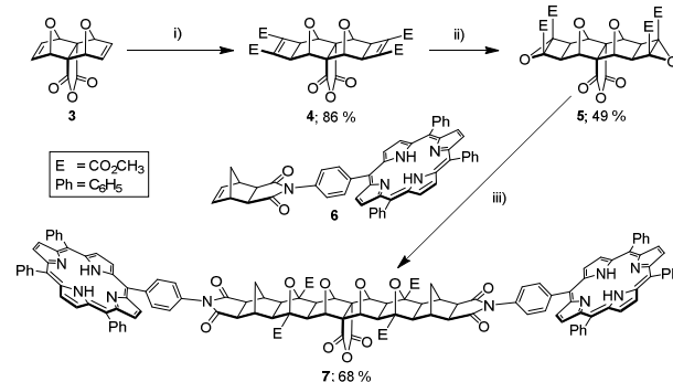
Figure 3. Convergent synthetic approach via bis-porphyrin anhydride 7 . i) DMAD (2-4 eq.), 5-20 mol-% [Ru(H_2CO)(PPh_3)_3] , toluene, 80 °C, N_2 atmosphere, 4 days, 86 %; ii) anhydrous 3.3 M t BuOOH in toluene (2.5 eq.), dry CH_2Cl_2 , 0 °C, N_2 atmosphere, 10 min, t BuOK (1 eq.), r.t., 3.5 hrs, 49 %; iii) exo -porphyrin receptor 6 (2 eq.), dry THF, microwave 80-220 W, 14-20 bar, 170 °C, 2 hrs, 68 %.
