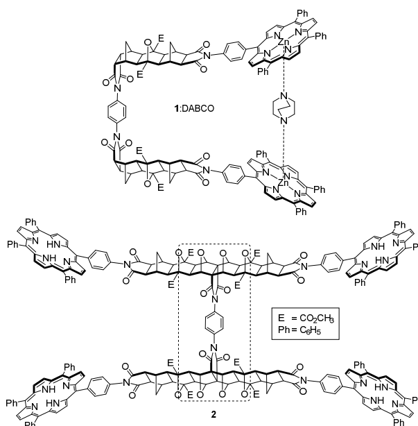
Figure 1. Previously described model tweezer system 1 11 (shown as complex with DABCO), and the expanded tetra-porphyrin molecular tweezer 2 with two bis-porphyrin binding sites linked via a bridged polycyclic scaffold and freely rotating phenyl diimide core (dotted line).
