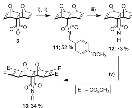
Figure 7. i) p -methoxybenzylamine (2 eq.), deacidified CHCl 3 , 50 °C, N 2 atmosphere, overnight; ii) NaOAc/Ac 2 O, 50 °C, N 2 atmosphere, overnight, 52 %; iii) 9:1 CH 3 CN/H 2 O, ammonium cerium(IV) nitrate (3 eq., 2 hrs; 2.3 eq. 90 mins + 0.3 eq. 30 mins), 40 °C, 73 %; iv) DMAD (4 eq.), 20 mol-% [Ru(H 2 CO(PPh 3 ) 3 )] 2 , dry DMF, 60 °C, N 2 atmosphere, 24 hrs, 34 %.
