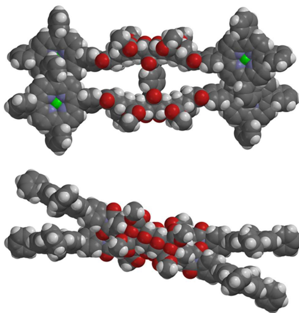
Figure 13. Molecular modelling of the zinc(II) metallated adduct of the two binding site tetra-porphyrin tweezer 2 in the absence of guest (side-on and top-down) (semi-empirical, AM1).
