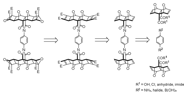
Figure 4. Retrosynthetic analysis of the phenyl diimide core.
