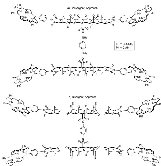
Figure 2. Schematic representations of convergent and divergent synthetic approaches to the synthesis of tetra-porphyrin tweezer 2 .
