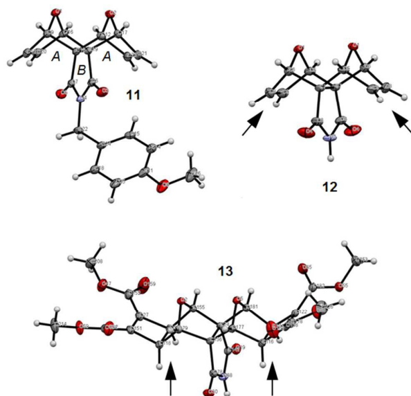
Figure 8. X-ray crystal structures of the imide series 11 , 12 and 13 . The arrows highlight the change in the position of the hydrogen atoms at the ring junctions following addition of the cyclobutene diester ring.
