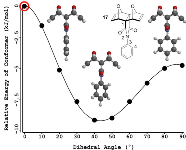
Figure 12. Rotational energy profile and barrier to rotation about the imide-phenyl single bond in a model of the linker, compound 17 (energy profile Hartree-Fock 6-31G*, energy of each conformation recalculated Density Functional B3LYP/6-31G*).
