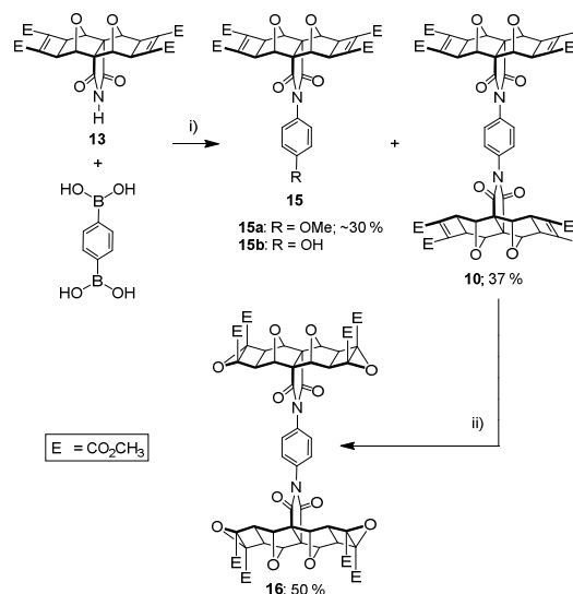
Figure 10. i) benzene-1,4-diboronic acid, copper(II) acetate (5 mol-%), MeOH or 9:1 THF/H 2 O, reflux, air bubbler, 18 hrs, ~30% 15a + 37% 10 ; ii) anhydrous 3.3 M tBuOOH in toluene (5 eq.), dry CH 2 Cl 2 , 0 °C, N 2 atmosphere, 10 min, tBuOK (2 eq.), r.t., 3.5 hrs, 50%.
