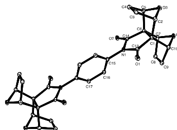
Figure 6. X-ray crystal structure of the centrosymmetric phenyl diimide core 9 . The DMSO molecules have been omitted for clarity, H atoms are not shown.
