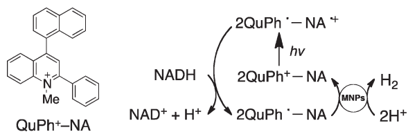
Scheme 1. Structure of QuPh + –NA and the Overall Catalytic Cycle for Photocatalytic Hydrogen Evolution Using QuPh + –NA and Metal Nanoparticles (MNPs, M = Ru, Pt, Fe)
