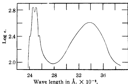
Fig. 1.—Ultraviolet absorption spectrum of pyridazine in hexane.
