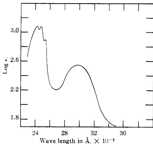
Fig. 2.—Ultraviolet absorption spectrum of pyridazine in water.
