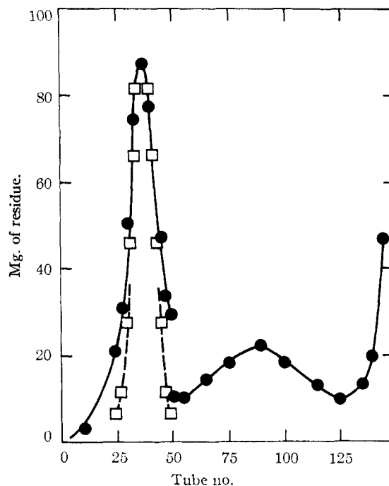
Fig. 3.—Countercurrent distribution of reaction products from treatment of acetylandromedol with acid. The solvent system used was prepared by mixing equal volumes of cyclohexane, ethyl acetate, ethanol and water. The operation was carried out with a 50 tube, 100 ml. per phase apparatus. Tubes 50 to 149 in the figure represent withdrawal fractions of top phase. The closed circles represent experimental points, and the calculated values for the theoretical curve are shown as open squares.
