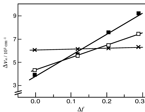
Fig. 4 Plot of difference between absorption and fluorescence wavenumber ( \Delta v_{\text{st}} ) vs. solvent polarity parameter ( \Delta f ) of 3 (x), 13 (□) and 15 (■) in cyclohexene (0.00), dipropyl ether (0.12), dichloromethane (0.21) and ethanol (0.29). Values in parentheses are \Delta f of each solvent.
