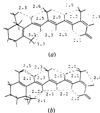
Fig. 2. Intramolecular H···H distances (Å). (a) 6- s-cis conformer. (b) 6- s-trans conformer. The 2.3 Å contact between H(7) and H(16 C ) is likely to be inaccurately short: note in Fig. 1 that H(16 C ) appears to be misplaced with respect to the remainder of its methyl group.
