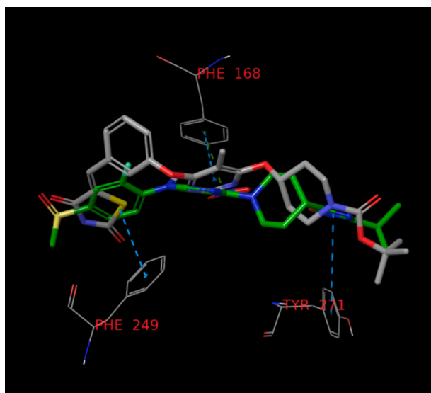
Fig. 9. AR 231453 (green) superposed with 13c (grey) in the GPR119 binding site. (For interpretation of the references to colour in this figure legend, the reader is referred to the web version of this article.)
