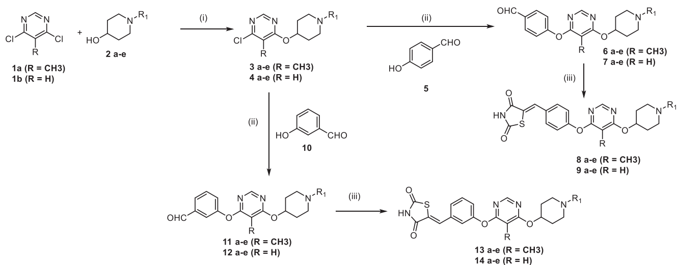
Scheme 1. Reagents and Conditions: (i) t -BuOK, THF, 0 °C, 30 min, (ii) K 2 CO 3 , DMA, 138 °C, 3 h, (iii) Thioazolidine-2,4-dione (TZD), Piperidine, benzoic acid, Toluene, Reflux, 7 h.
