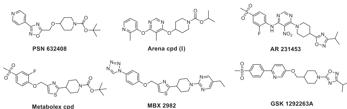
Fig. 1. The synthetic ligands of GPR119 Agonists.
