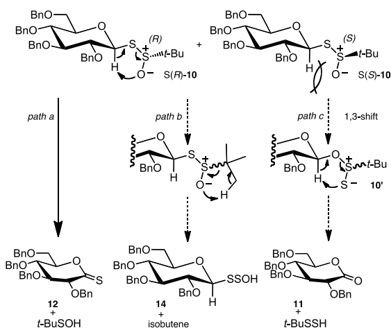
Scheme 3: Possible reaction paths for the thermolysis of D-glucosyl tert -butyl thiosulfates 10
