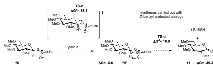
Figure 2. 1,3 Shift of the thiosulfinate group in 10 , followed by E1 elimination ( path c ). \Delta G in kcal.mol -1
