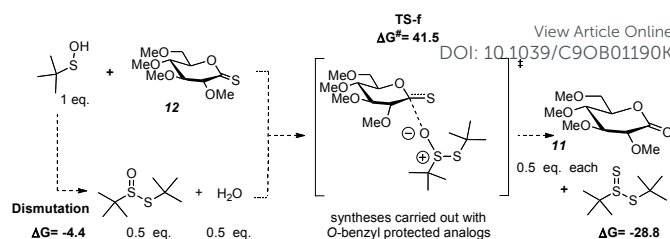
Figure 4. Dismutation of tert -butyl sulfenic acid, and di- tert -butyl thiosulfinate attacking thionolactone 12 . \Delta G in kcal.mol -1
