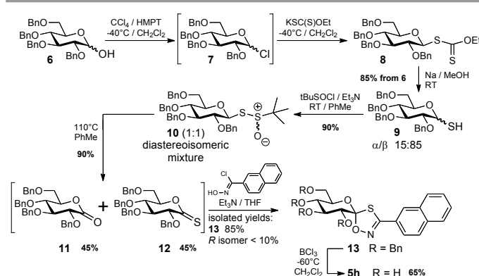
Scheme 2. New access to 15-glucopyranosylidene-spiro-oxathiazole by nitrile oxide-thionolactone 1,3-dipolar cycloaddition
