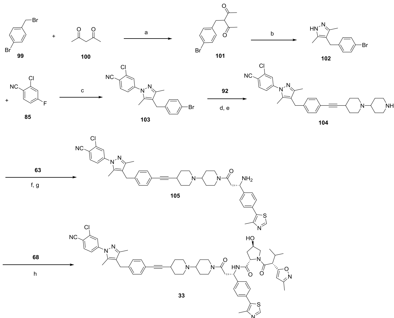
Scheme 8. Compound 33 a
