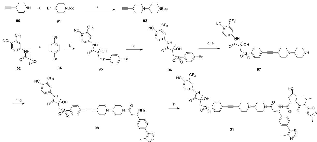
Scheme 7. Compound 31 a
