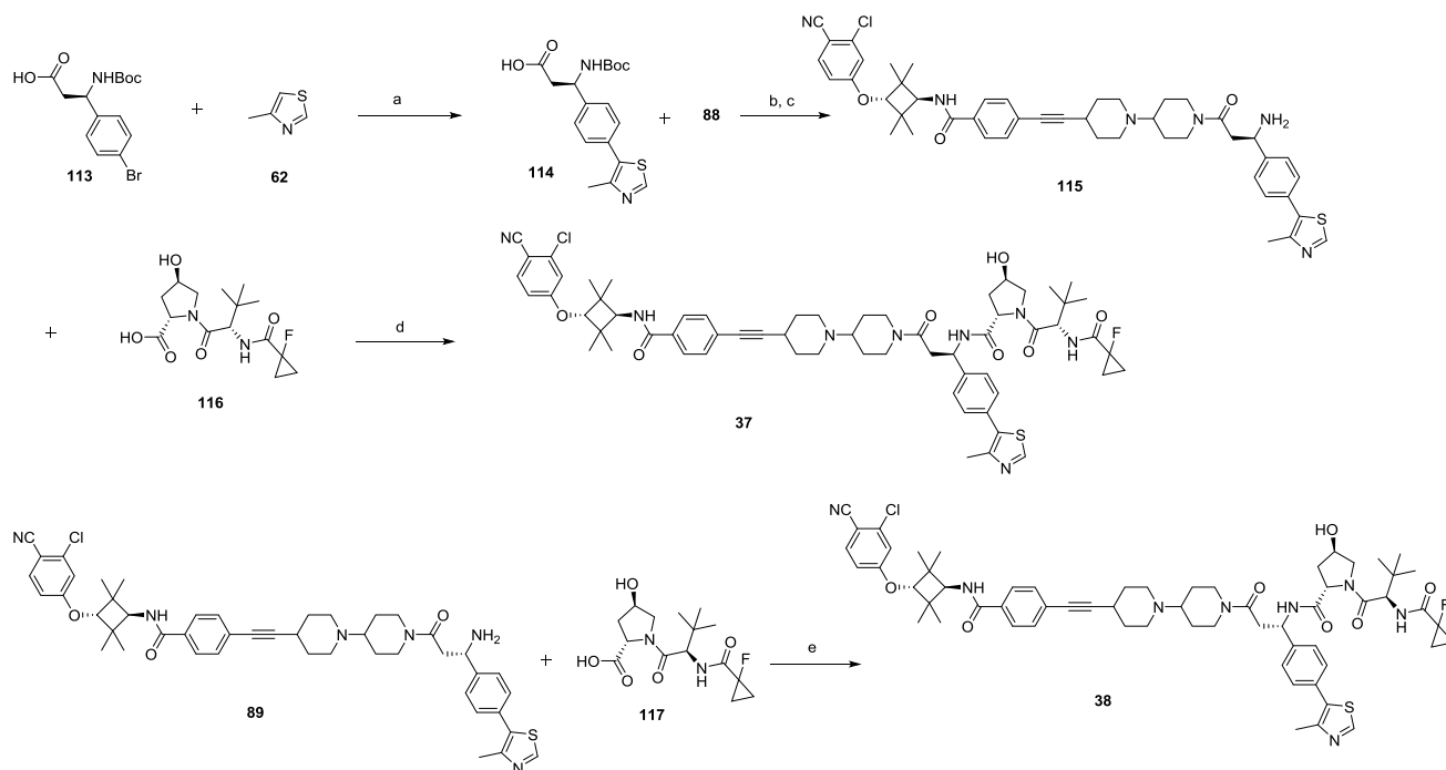
Scheme 10. Compounds 37–38 a
