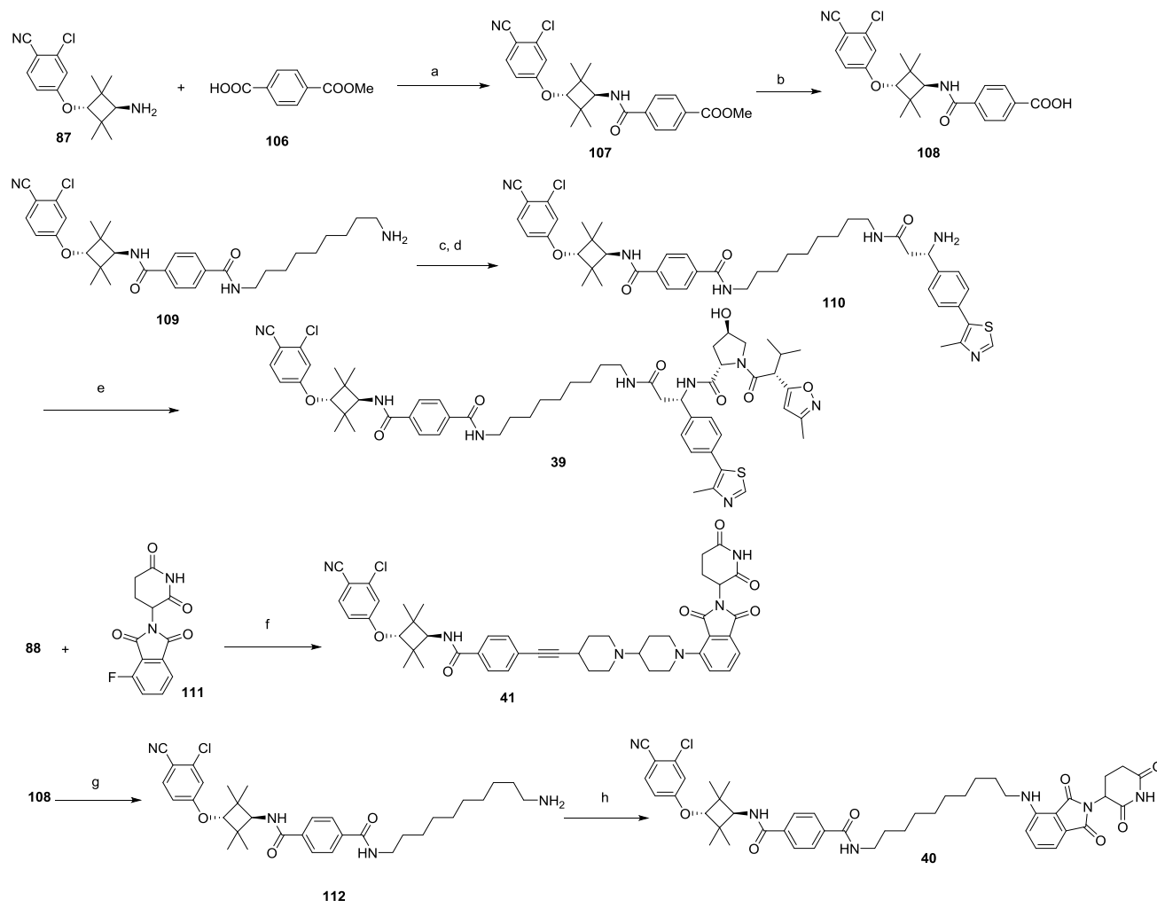
Scheme 9. Compounds 39–41 a
