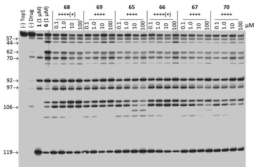
Figure 3. Top1-mediated DNA cleavage assay gel: lane 1, DNA alone; lane 2, DNA and Top1; lane 3, DNA and Top1 and 1 \mu M camptothecin (1); lane 4, DNA and Top1 and 1 \mu M MJ-III-65 (6); lanes 5–28, DNA and Top1 and indicated concentration ( \mu M) of test compound. The numbers and arrows at the left indicate cleavage site positions (see Experimental Section). Gel-based assays are commonly acquired twice for each compound, and they are always run with positive controls, including camptothecin and an indenoisoquinoline.
