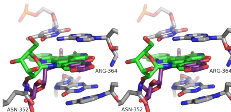
Figure 7. Overlay of 10 (green) and 62 (purple) within the X-ray crystal structure of a stalled Top1–DNA cleavage complex cocrystallized with 9 (PDB code 1SC7). The stereoview is programmed for wall-eyed (relaxed) viewing.
