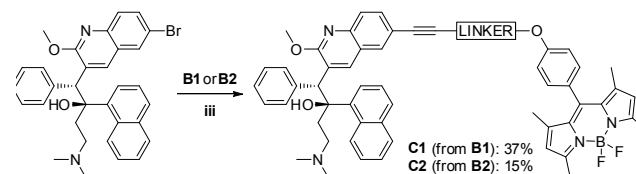
Figure 5: Labeling of Bedaquiline using a Sonogashira Coupling. Reaction conditions: iii. Bedaquiline fumarate 1 eq, BODIPY 1.5 eq, CuI 0.05 eq, Pd(PPh 3 ) 4 0.2 eq in 10 mL 1:1 DMF:NEt 3 added under Argon atmosphere at rt; reaction heated at 90 °C for 2h.
