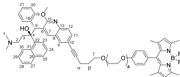
Figure 3: Structural formula of Bedaquiline-pentynoxy-eg 4 -BODIPY C2 . The numbering scheme used in this work for elucidation of NMR spectroscopic data is shown.
