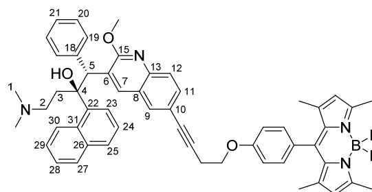
Figure 2: Structural formula of Bedaquiline-butynyloxy-BODIPY. The numbering scheme used in this work for elucidation of NMR spectroscopic data is shown.
