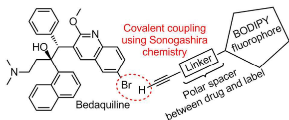
Figure 1: Structural formula of Bedaquiline and schematic depiction of fluorescent label. Using a Sonogashira cross-coupling, the alkyne-terminated polar linker attached to the BODIPY fluorophore will be covalently coupled to the aryl bromide position of Bedaquiline.
