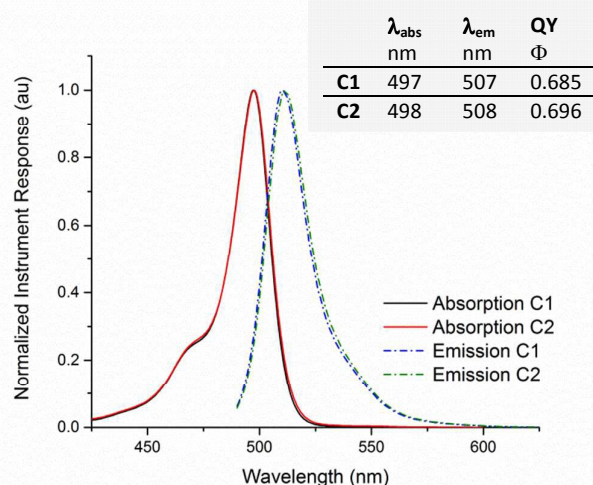
Figure 6: Emission and Absorption curves for compounds C1 and C2. Normalized absorption (solid lines) and emission (dashed lines) plots, recorded in acetonitrile solution. The inset tabulates absorption and emission wavelength maxima \lambda_{\text{abs}} and \lambda_{\text{em}} and the corresponding quantum yield of fluorescence \Phi , calculated using fluorescein in 0.1 M aqueous NaOH as a reference. Peak normalized instrument responses for absorption measurements correspond to an extinction coefficient of respectively \epsilon = 7.6 \cdot 10^3 ( C1 ) or 6.8 \cdot 10^3 ( C2 ) cm 2 mol -1 .
