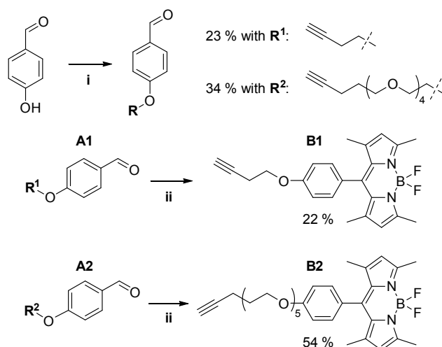
Figure 4: Synthesis of alkyne-functionalized BODIPY derivatives. Reaction conditions: i. 4-hydroxybenzaldehyde (1 eq.), alcohol R 1 -OH or R 2 -OH (1 eq.), PPh 3 (1.05 eq.), DEAD (40 wt% in toluene, 1 eq.), THF, 0 °C → rt, overnight; ii. A (1 eq.), 2,4-dimethylpyrrole (2.2 eq.), TFA (cat.), THF, rt, 16h; then DDQ 1 eq.), rt, 1h; then NEt 3 (excess), BF 3 ·OEt 2 (excess), 0 °C → rt, 2h.
