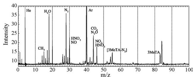
Fig. 13. Mass spectrum from rapid thermolysis of Me1ATN at 340 °C and 1 atm Ar, He and residual air (average of 10 spectra).
