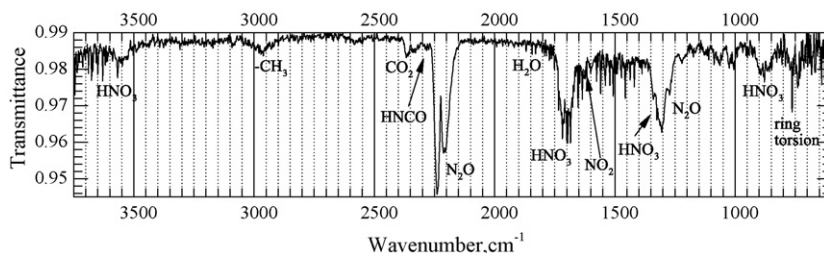
Fig. 12. FTIR spectrum of species from rapid thermolysis of Me1ATN at 340 °C and 1 atm N 2 .
