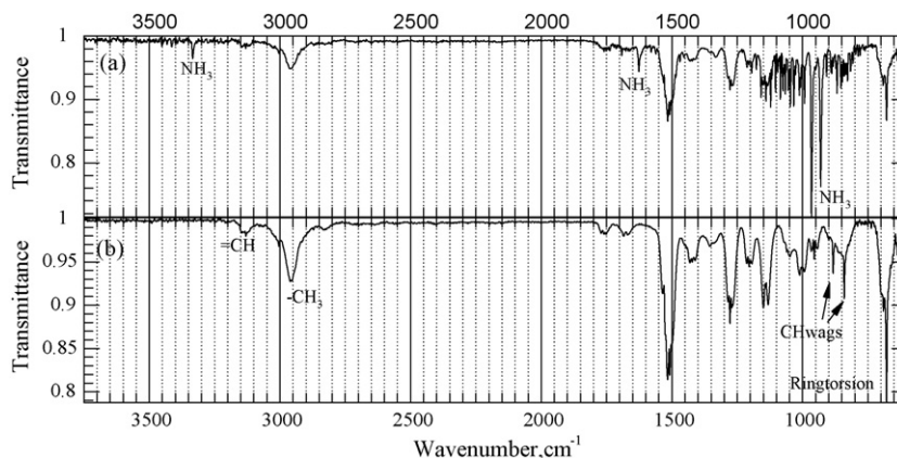
Fig. 2. FTIR spectrum of species from rapid thermolysis of (a) Me4ATI at 270 °C and 1 atm N 2 , and (b) MeTA at 250 °C and 1 atm N 2 .
