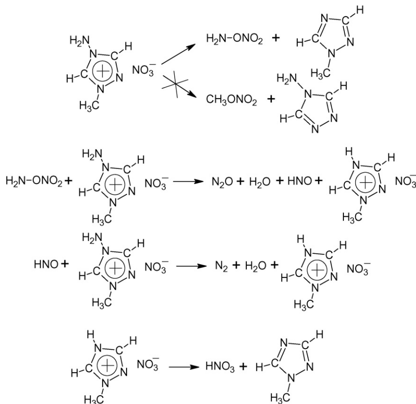
Scheme 2. Proposed reaction pathway for Me4ATN.
