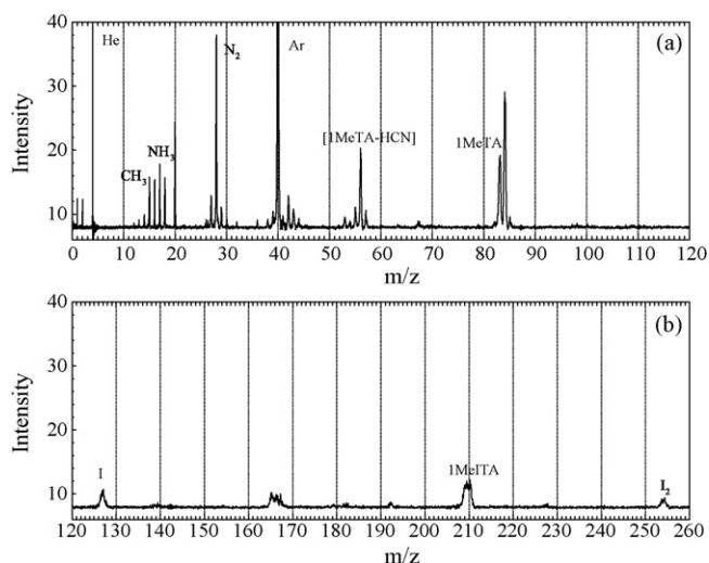
Fig. 3. Mass spectrum from rapid thermolysis of Me4ATI at 270 °C and 1 atm Ar, He and residual air (average of 10 spectra).
