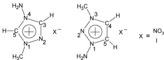
Fig. 1. Structure of 1-methyl-4-amino-1,2,4-triazolium X (X = iodide and nitrate) and 1-amino-3-methyl-1,2,3-triazolium X (X = iodide and nitrate).
