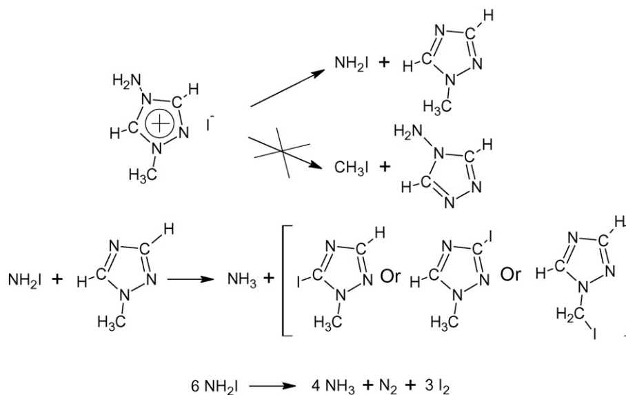
Scheme 1. Proposed reaction pathway for Me4ATI.
