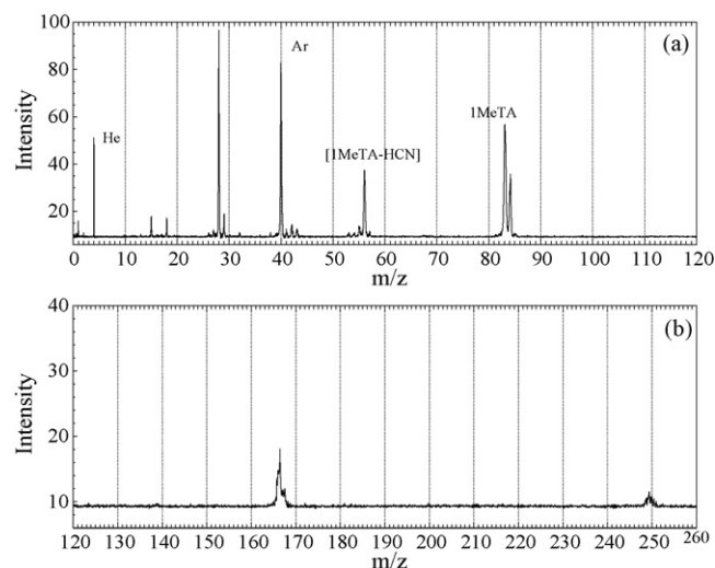
Fig. 4. Mass spectrum from rapid thermolysis of MeTA at 250^\circ\text{C} and 1 atm Ar, He and residual air (average of 10 spectra).
