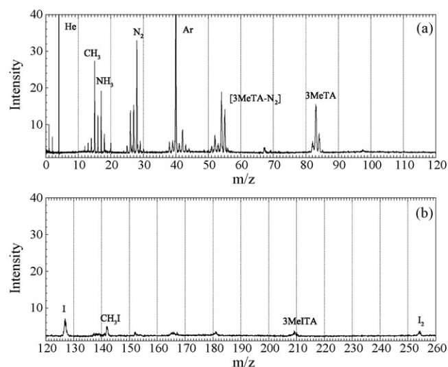
Fig. 9. Mass spectrum from rapid thermolysis of Me1ATI at 290 °C and 1 atm Ar, He and residual air (average of 10 spectra).
