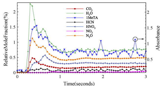
Fig. 7. Species evolution from rapid thermolysis of Me4ATN at 320 °C and 1 atm N 2 .
