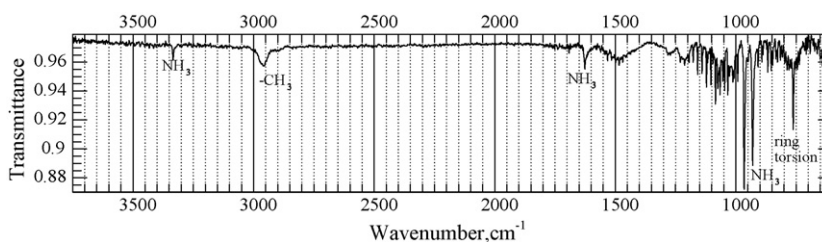
Fig. 8. FTIR spectrum of species from rapid thermolysis of Me1ATI at 290 °C and 1 atm N 2 .
