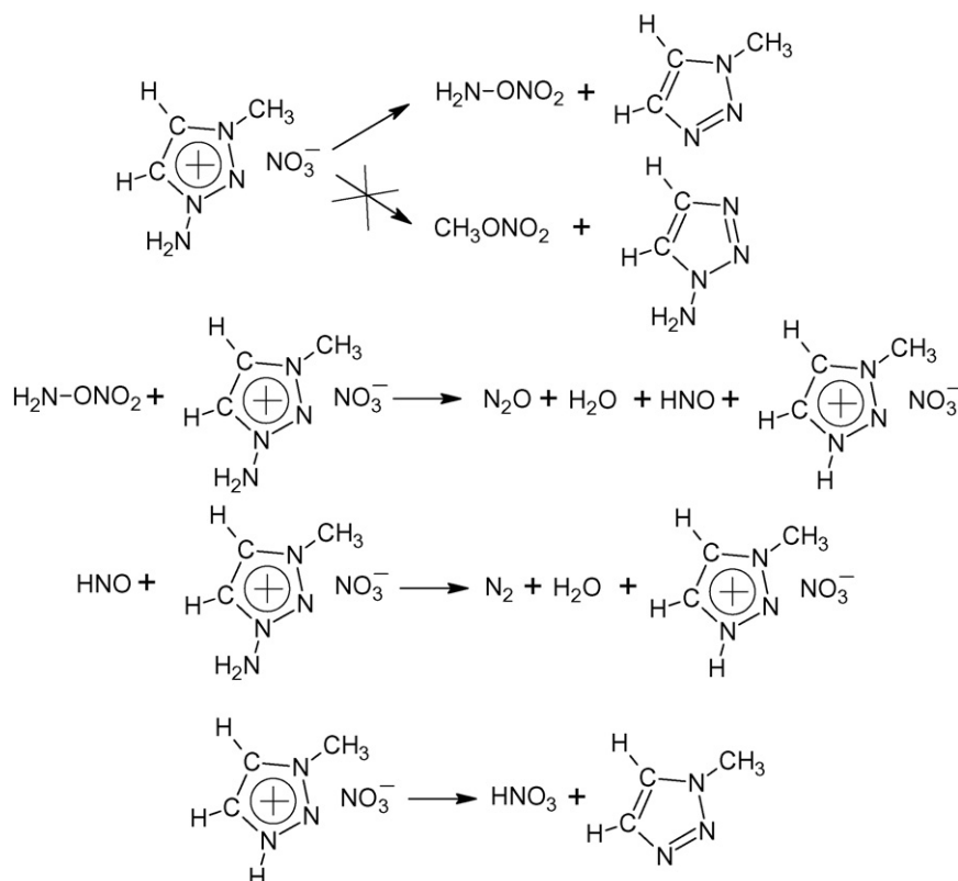
Scheme 4. Proposed reaction pathway for Me1ATN.
