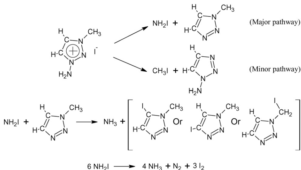
Scheme 3. Proposed reaction pathway for Me1ATL.
