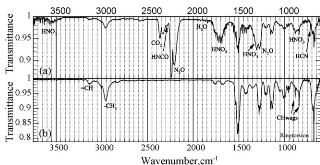
Fig. 5. FTIR spectrum of species from rapid thermolysis of (a) Me4ATN at 320 °C and 1 atm N 2 , and (b) MeTA at 250 °C and 1 atm N 2 .
