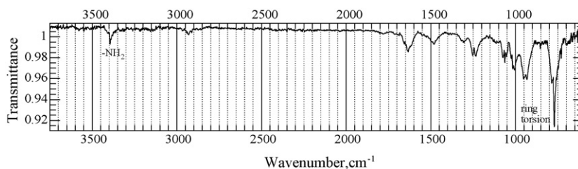
Fig. 10. FTIR spectrum of species from rapid thermolysis of 1ATA at 350 °C and 1 atm N 2 .
