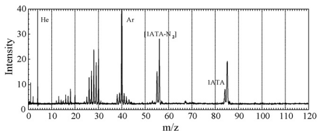
Fig. 11. Mass spectrum from rapid thermolysis of 1ATA at 350 °C and 1 atm Ar, He and residual air (average of 10 spectra).
