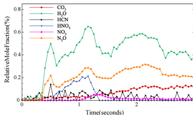
Fig. 14. Species evolution from rapid thermolysis of Me1ATN at 340 °C and 1 atm N 2 .
