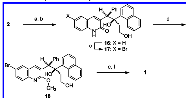
Scheme 3. Completion of the Synthesis a
