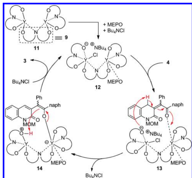
Scheme 2. Proposed Model of the Catalytic Cycle
