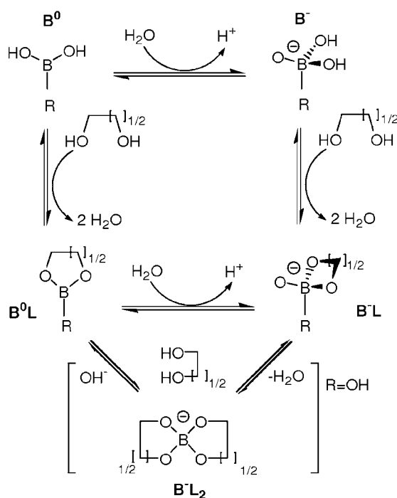
Scheme 2. Ester formation between 1,2- or 1,3-diols and boric acid ( R = OH ) or phenylboronic acid ( R = Ph ).
