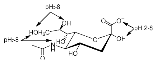
Figure 8. Schematic representation of the possible binding sites for PBA on Neu5 Ac.
