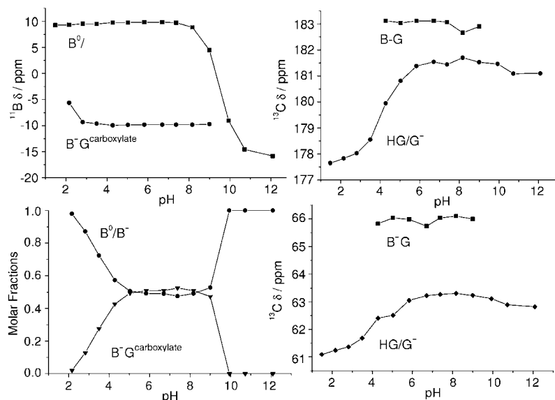
Figure 1. pH dependence of the ^{11}\text{B} NMR resonances (top left), molar fractions calculated from the integration of the ^{11}\text{B} NMR resonances (bottom left), and pH dependence of the ^{13}\text{C} NMR resonances in the carbonyl (top right) and aliphatic area (bottom right) for a mixture of glycolic acid (1M) and phenylboronic acid (1M).
