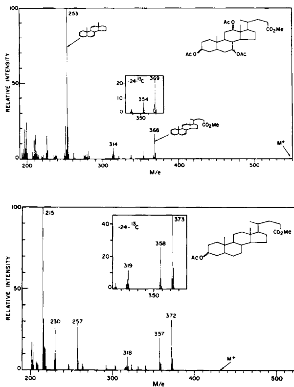
Figure 3. Mass spectra of bile acids: cholic acid (top) lithocholic acid (bottom).
