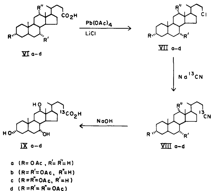
Figure 2. Synthesis of 24- ^{13}\text{C} labeled bile acids.
