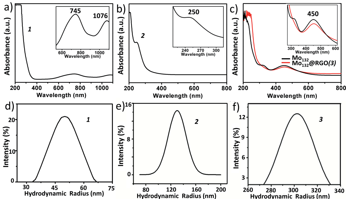
Fig. 4 UV-Vis spectroscopy of 1, 2 and 3 (upper panel) shows characteristic bands for \{Mo_{154}\} (745 and 1076 nm), \{Mn_6P_3W_{24}\} (250 nm) and \{Mo_{132}\} (450 nm). The magnified characteristics bands are shown in the insets. The lower panel represents the hydrodynamic radius obtained from DLS spectroscopy of 1, 2 and 3 with an average of 51, 130 and 300 nm, respectively.
