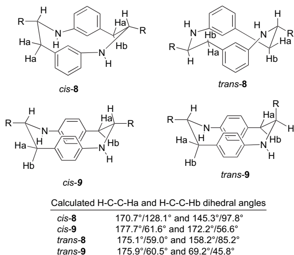
Figure 2. Side view of cis - and trans -diastereoisomer of metacyclophane ( 8 ) and paracyclophane ( 9 ).
