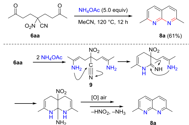
Scheme 6. A concise construction of [1,8]-naphthyridine 8 via double cyclization/aromatization procedure from diketone 6aa .
