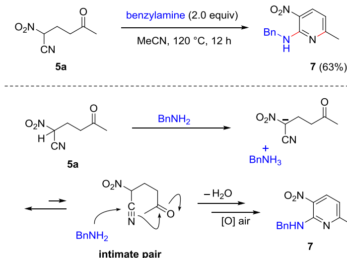
Scheme 5. Synthesis of vicinally functionalized pyridine 7 from single adduct 5a via pseudo-intramolecular process.
