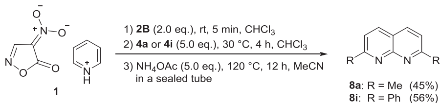
Scheme 7. Synthesis of [1,8]-naphthridine 8 from the pyridinium salt of nitroisoxazalone 1 .
