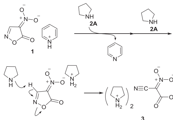
Scheme 1. Generation of cyano- aci -nitroacetate 3 derived from nitroisoxazalone 1 .
