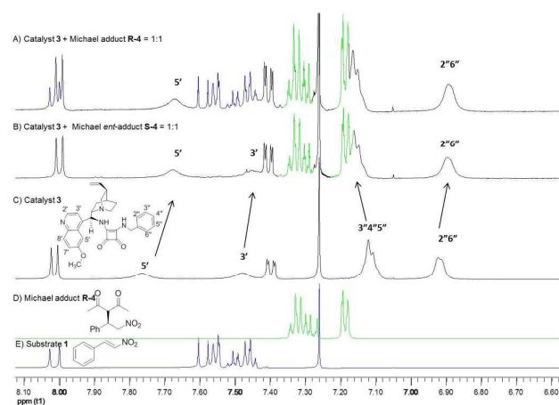
Fig. 8 NMR complexation studies of the R-4 or S-4 Michael adducts-catalyst mixtures.
