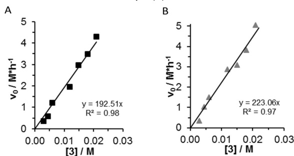
Fig. 3 Initial reaction rate vs. catalyst (3) concentration by two sets of experiments. A) in the case of nucleophile excess, square: [1]_0 = 0.3 M; [2]_0 = 0.6 M; [3] = 0.003 - 0.021 M; B) in the case of electrophile excess, triangle [1]_0 = 0.6 M; [2]_0 = 0.3 M; [3] = 0.003 - 0.021 M.
