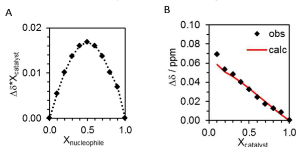
Fig. 4 A) Curve-fitting on measured chemical shifts-difference. B) Plot of weighted ^1\text{H} -NMR shifts versus mole fraction and the calculated complex concentrations versus mole fraction.
