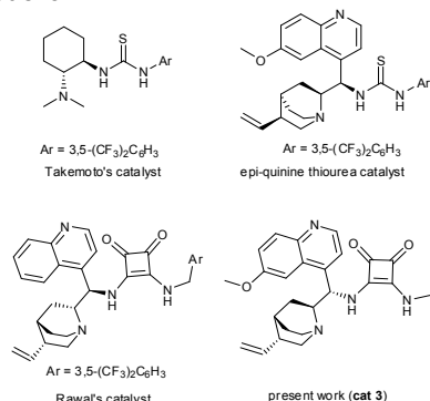
Scheme 1 Bifunctional thiourea- and squaramide-based organocatalysts.
