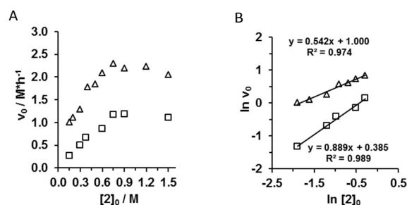
Fig. 5 Determination of reaction order in acetylacetone (2), A) initial reaction rate vs. initial concentration of (2), [2]_0 = 0.15 - 1.5 M, [3] = 0.006 M, square [1]_0 = 0.3 M, triangle [1]_0 = 0.6 M, B) natural logarithm of initial reaction rate.
