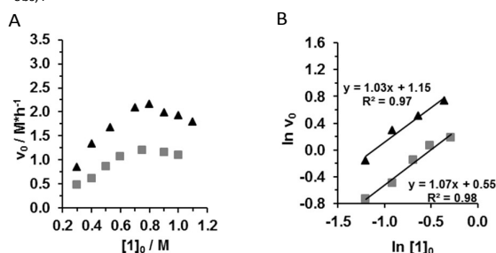
Fig. 6 Determination of order in \beta -nitrostyrene ( 1 ), A) initial reaction rate vs. initial concentration of ( 1 ), [1]_0 = 0.3 - 1.1 M, [3] = 0.006 M, square [2]_0 = 0.3 M, triangle [2]_0 = 0.6 M; B) natural logarithm of initial reaction rate.
