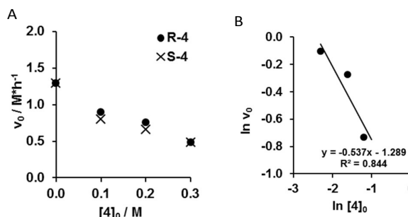
Fig. 7 A) Initial reaction rate at different initial product (circle R-4 , or \times S-4 ) concentration, [1]_0 = 0.6 M; [2]_0 = 0.3 M, [3] = 0.006 M; B) natural logarithm of initial reaction rate in the presence R-4 .
