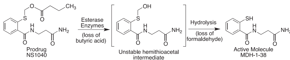
Fig. 2. Cleavage of NS1040 to MDH-1-38 by cellular esterases.
