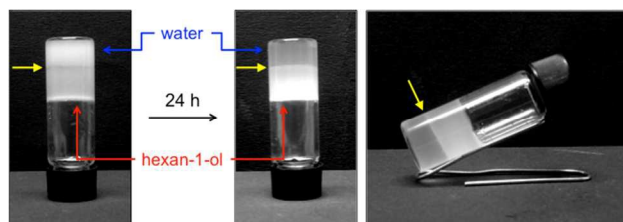
Fig. 3 Phase-selective gelation and change in opacity of hexan-1-ol/water mixture after 24 h (gelator 1 , c = 7 g L -1 ). Total volume = 2 mL. Yellow arrow indicates the boundary between phases.
