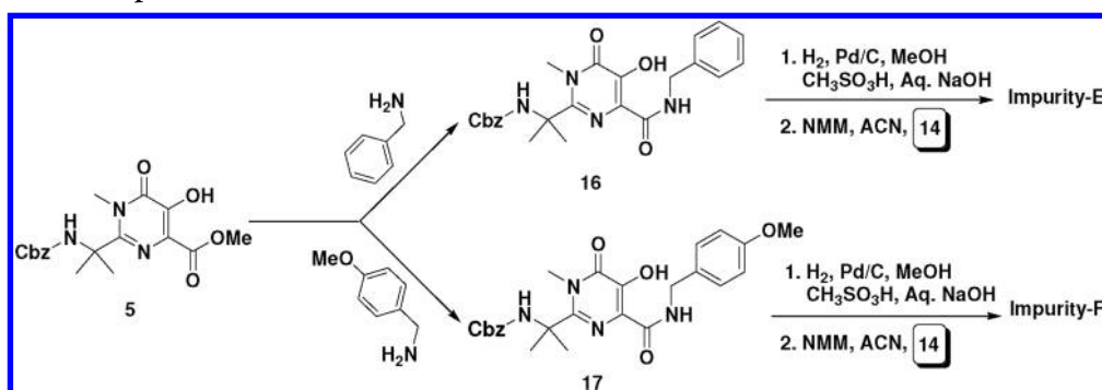
Scheme 6. Synthesis of impurities E and F
