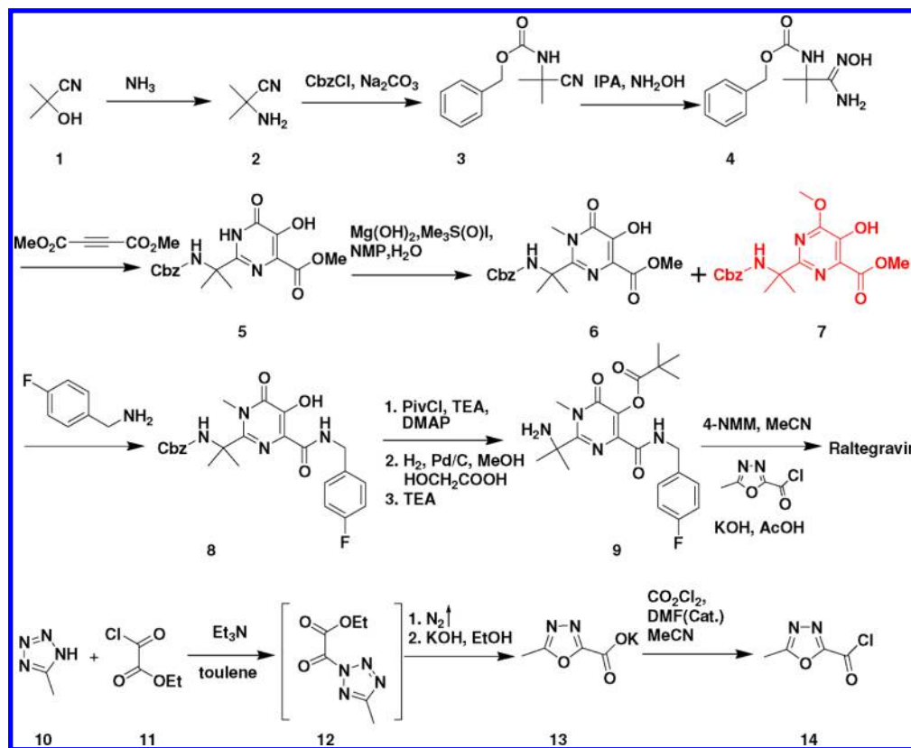
Scheme 2. Amide disconnection
