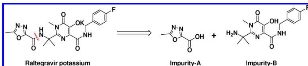
Scheme 2. Amide disconnection
