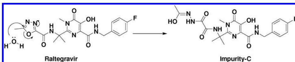
Scheme 5. Synthesis of impurities D and G
