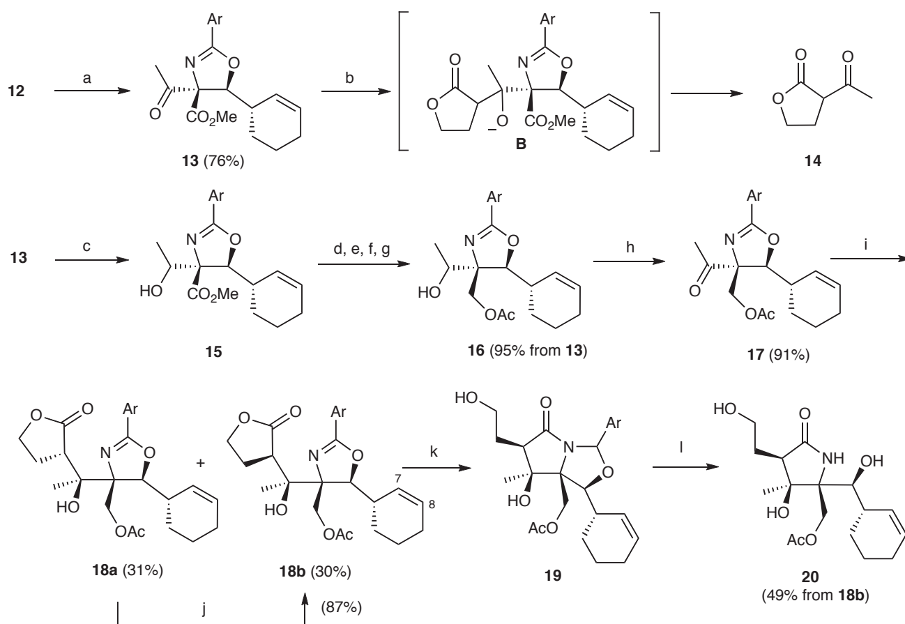
Scheme 3. Synthesis of \gamma -lactam 20 . Reagents and conditions (Ar = p -Cl-C 6 H 4 -): (a) n -BuLi (2 equiv), i -Pr 2 NH (2.2 equiv), THF, -78 °C; AcCl (3 equiv), 15 min; (b) \gamma -butyrolactone, LDA, THF, -78 °C; (c) NaBH 4 (1.5 equiv), MeOH, -40 °C, 2 h; (d) DHP (5 equiv), PPTS (0.22 equiv), CH 2 Cl 2 , reflux, 3 h; (e) DIBALH (3 equiv), THF, -5 °C, 9 h; (f) Ac 2 O (3 equiv), Et 3 N (6 equiv), DMAP (0.1 equiv), CH 2 Cl 2 , reflux, 3 h; (g) Me 2 AlCl in hexane (2 equiv), CH 2 Cl 2 , 0 °C to rt, 0.5 h; (h) 1-Me-AZADO (0.11 equiv), PhI(OAc) 2 (1.65 equiv), CH 2 Cl 2 , rt, 12 h; (i) (Ph 3 P) 3 RhCl (0.05 equiv), \alpha -bromo- \gamma -butyrolactone (4 equiv), Et 2 Zn (4 equiv), THF, -20 °C, 3 h; (j) DBU (1.1 equiv), CH 2 Cl 2 , 0 °C, 12 h; (k) NaBH 3 CN (5 equiv), AcOH-THF (2:1), 0 °C, 6 d; (l) 1,2-propanedithiol (4.2 equiv), cHCl, CF 3 CH 2 OH, rt, 0.5 h.
