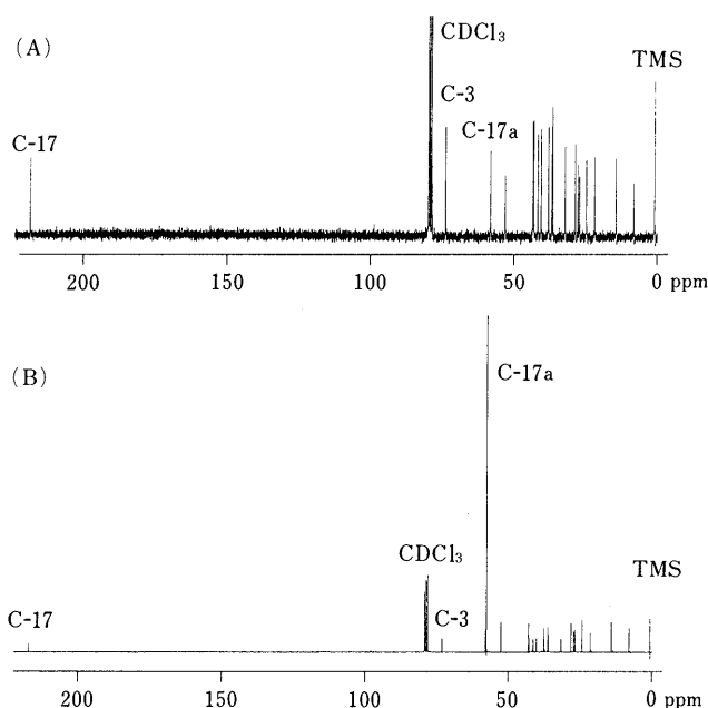
Fig. 2. 13 C-NMR Spectrum of (A) 3α-Hydroxy-17αβ-methyl-D-homo-5β-androstan-17-one ( 13a ) and That of (B) the Degradation Product of [20- 13 C]-Pregnane-3α,17α,20α-triol 20-Sulfate ( 8b )
