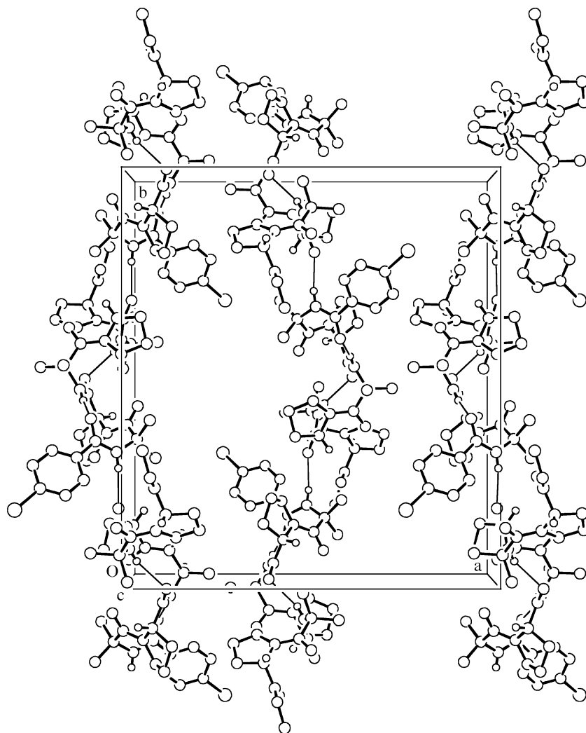
Fig. 3. Packing diagram of 11 showing the H-bonding interactions (uninvolved H-atoms omitted for clarity)
