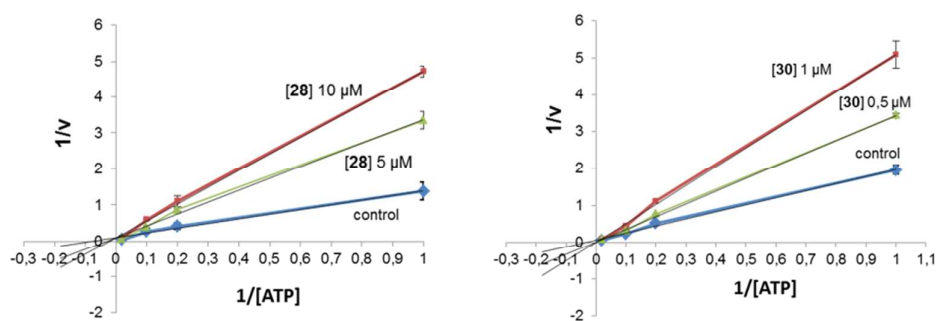
Figure 5. Kinetic data for the TZD-derivatives 28 and 30 . ATP concentration in the reaction mixture varied from 1 to 50 \mu M . Compounds concentrations used are depicted in the plot, and the concentration of GS-2 was kept constant at 25 \mu M . Each point is the mean of two different experiments, both analyzed in triplicate.
