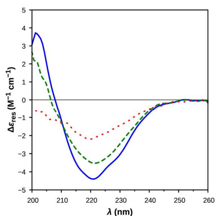
Figure 8. CD spectra of AcPHF6 (100 \mu M) in the absence ( solid ) and in the presence of 28 (20 \mu M, dashed ) or 30 (20 \mu M, dotted ), measured after 2 h incubation. Solvent: phosphate buffer (50 mM pH 7.4)/water/methanol/DMSO 89:10:0.95:0.05 (v/v/v/v). Pathlength: 1 mm.
