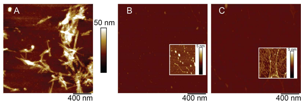
Figure 9. AFM micrographs of amyloid fibers obtained from the aggregation of 50 \mu M AcPHF6 peptide in phosphate buffer in the absence (A), and in the presence of 10 \mu M compound 28 (B) and
