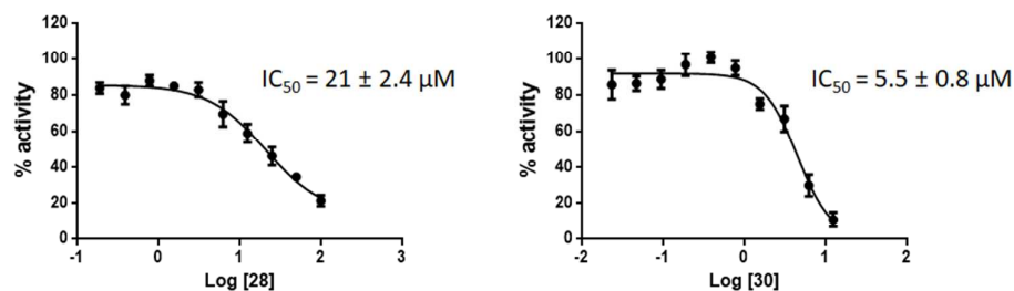
Figure 4. Dose-response curves of GSK-3β activity in the presence of 28 and 30 . Values are the means \pm SD determined for at least two independent experiments.
