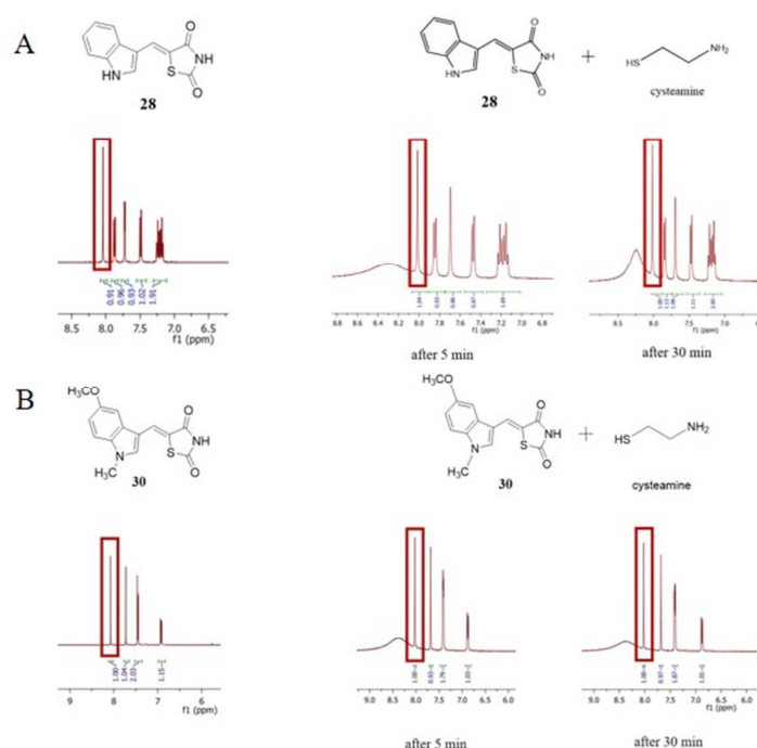
Figure 14. Thiol trapping assay. 1 H-NMR spectrum of 28 (A) and 30 (B) in DMSO- d 6 and in DMSO- d 6 with cysteamine (1:2). In the squares, the olefin signal is highlighted. No reaction occurs, even after 30 minutes.
