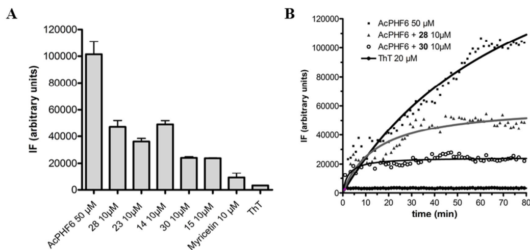
Figure 7. (A) Inhibition of AcPHF6 peptide (50 \mu M) aggregation in the presence of selected derivatives (10 \mu M) after 80 min incubation. The data are the mean of at least three repeats. (B)
