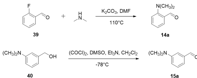
Scheme 2. Synthetic procedure for the synthesis of aldehydes 14a and 15a .
