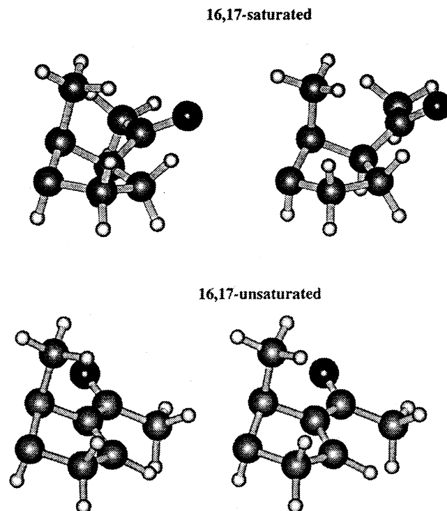
Fig. 3. Preferred conformations of epalon derivatives. Stereodiameter of the D-ring of 3\alpha -hydroxy- 5\alpha -pregnan-20-one ( 3\alpha,5\alpha -P)(epiallopregnanolone) and 3\alpha -hydroxy- 5\alpha -pregn-16-en-20-one ( 3\alpha,5\alpha -16-en-P) showing the preferred orientation of the 20-keto group in each case.
