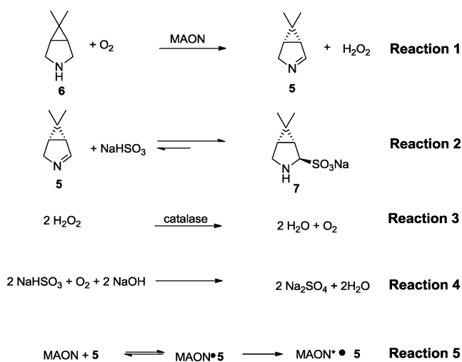
Scheme 3. List of Reactions in Amine Oxidation and Imine Sulfonations Cascade
