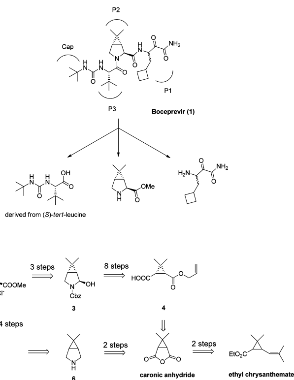
Scheme 1. Key Disconnections in Boceprevir and the Retro-Synthesis of the Central P2 Moiety
