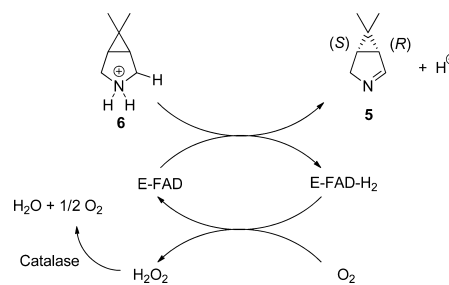
Scheme 2. Mechanism for Monoamine Oxidase-Catalyzed Oxidation of 6,6-Dimethyl-3-azabicyclo[3.1.0]hexane
