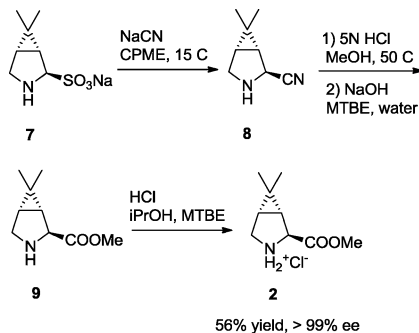
Scheme 4. Preparation of the P2 Intermediate from 7
