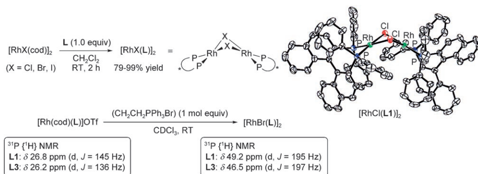
Scheme 2. Preparation of halogen-bridged dimeric Rh-phosphine complexes [RhX(L)]_2 .
