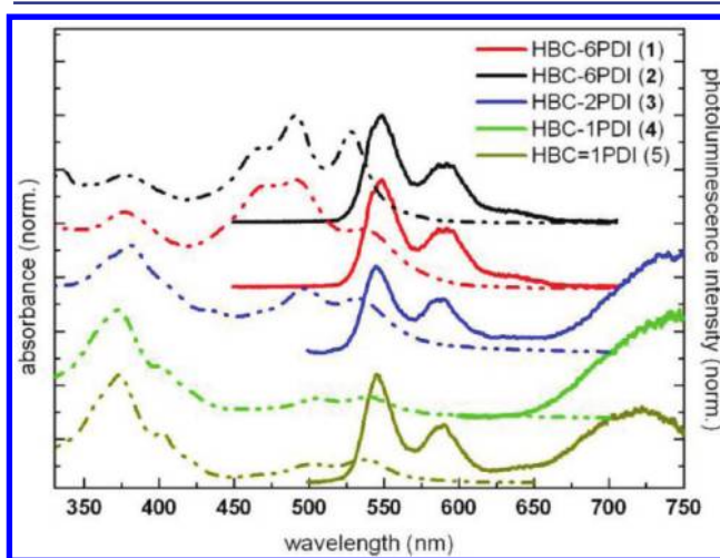
Figure 4. Normalized absorption (dashed lines) and emission spectra (solid lines) of dyads 1–5 in toluene, each at a concentration of 10^{-5} mol/L. For photoluminescence measurements HBC moieties were selectively excited at 375 nm with a 100 fs laser pulse.
