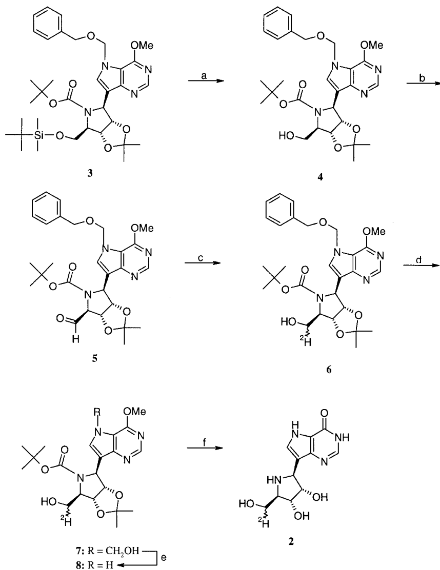
Scheme 1. Reagents and conditions: a. tetrabutylammonium fluoride, THF, ice-water bath; b. Dess-Martin periodinane, CH 2 Cl 2 , rt; c. NaB[ 2 H] 4 , CH 3 OH[ 2 H]; d. H 2 , 20% Pd(OH) 2 /C, EtOH; e. trace NH 4 OH; f. HCl, MeOH, reflux
