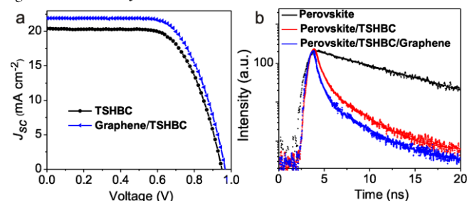
Figure 3. The best I-V characteristics of the cells (a), the transient PL spectra of films (b), based on 20 nm HTM layers.
