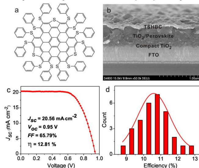
Figure 1. (a) The structures of TSHBC. (b) Cross-sectional SEM image of the device of FTO/TiO 2 /perovskite/TSHBC film. The best I-V characteristics (c), comparison of the performance distributions of 30 individual devices (d) of the cells.
