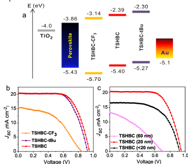
Figure 2. (a) The energy level diagram of the materials used in PSCs. (b) The best I-V characteristics of the cells. (c) The best I-V characteristics of the cells based on TSHBC with different thickness.
