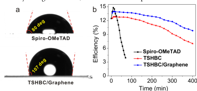
Figure 4. (a) The water contact angles. (b) The efficiency variation of the devices stored under illumination at AM 1.5 G with the humidity of 45%.
