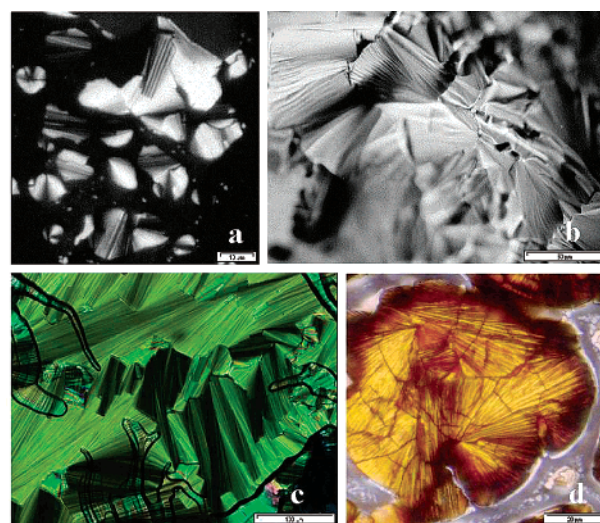
Figure 2. (a) Optical micrograph between crossed polarizers of 1b after annealing at 400 °C for 72 h; scale bar 10 \mu m. (b) Surface of the same sample imaged with differential interference contrast in reflected light; scale bar 50 \mu m. (c) Optical micrograph of 1b between crossed polarizers after short annealing at 400 °C; scale bar 100 \mu m. (d) Optical micrograph of 1b between crossed polarizers after prolonged annealing for 72 h at 400 °C; scale bar 20 \mu m. The micrographs were recorded at room temperature.
