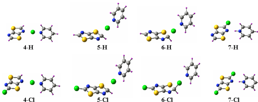
Figure 4. Optimized structures of stationary points for the pyridine-catalyzed chlorination of thiazolo[5,4- d ]thiazole 1 and 2-chloro-thiazolo[5,4- d ]thiazole 2a , according to the direct C-chlorination mechanism. Structures shown in the figure are from B3LYP/6-31+G(d) optimizations.
