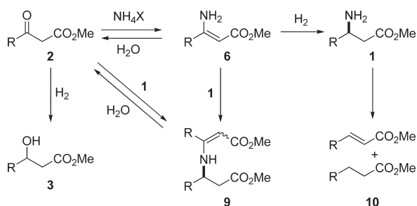
Scheme 4. Plausible mechanism for the asymmetric reductive amination of \beta -keto esters
