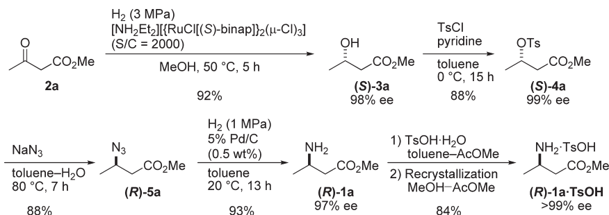
Scheme 2. Synthetic route via an azide compound
