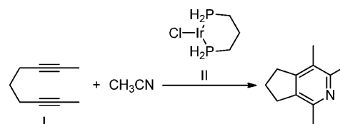
Scheme 6
