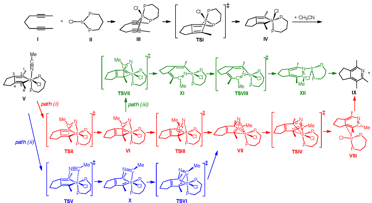
Scheme 7
