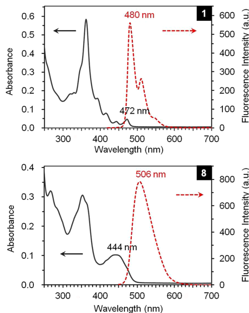
Figure 2. Absorption and fluorescence (excited at 410 and 440 nm, respectively) spectra of 1 (top) and 8 (bottom) in CH_2Cl_2 ( 5 \times 10^{-6} mol/L).
