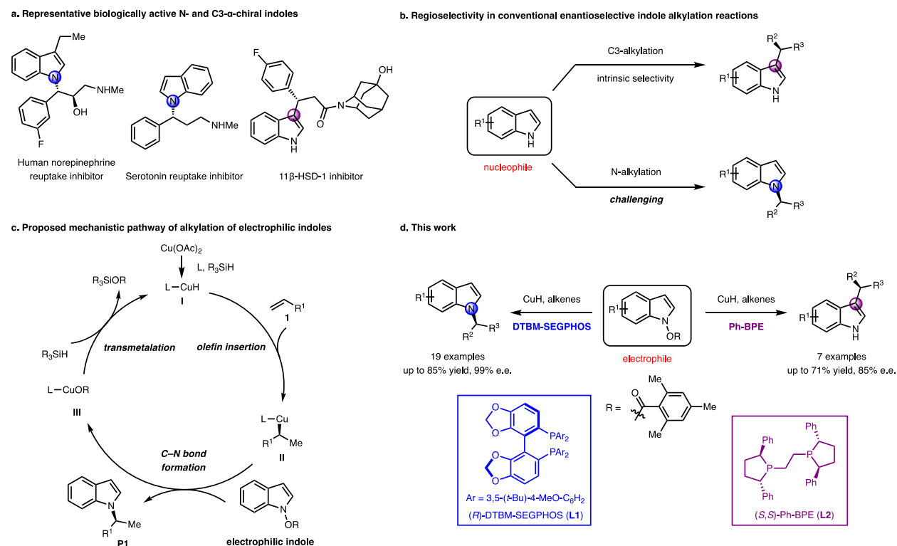
Figure 1. Design of a CuH-catalyzed indole alkylation reaction using electrophilic indole reagents. a) Representative biologically active N- and C3-substituted \alpha -chiral indoles. b) Regioselectivity in conventional enantioselective indole alkylation reactions. c) Proposed mechanistic pathway of enantioselective alkylation of electrophilic indoles. d) Ligand-controlled regiodivergent alkylation of electrophilic indoles.
