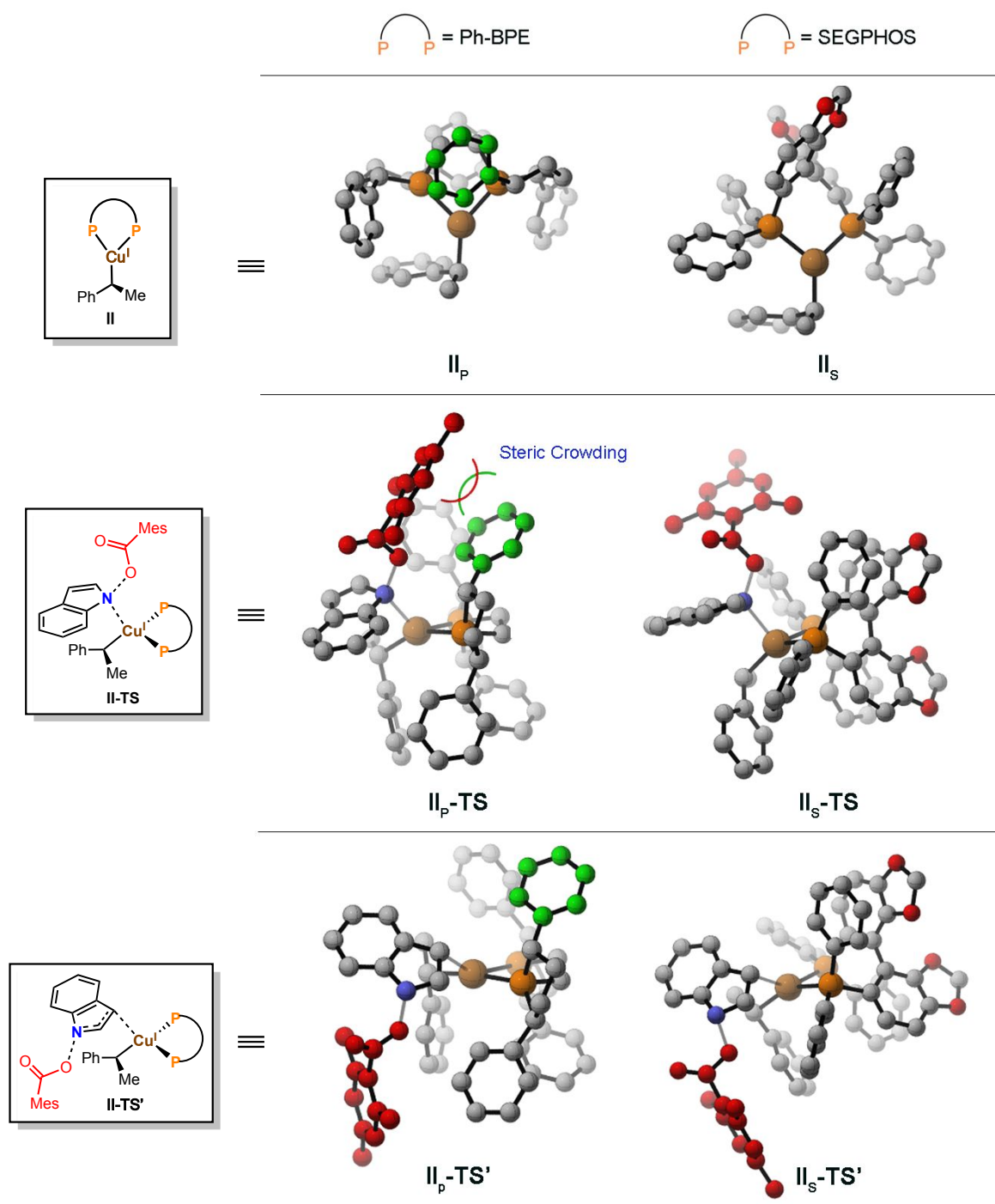
Figure 2. DFT calculations on the mechanism of CuH-catalyzed alkylation of electrophilic indoles. a) Proposed regiochemistry-determining reaction pathway. The mesitoate anion is omitted for clarity in the many of the structures. b) Energy profiles of the oxidative addition and reductive elimination steps with 2d and alkylcopper(I) complex II supported by SEGPLIOS and Ph-BPE, respectively. c) The optimized structures of II , II-TS , and II-TS' with Ph-BPE and SEGPLIOS as the ligand, respectively. The phenyl group in the Ph-BPE ligand obscuring the
