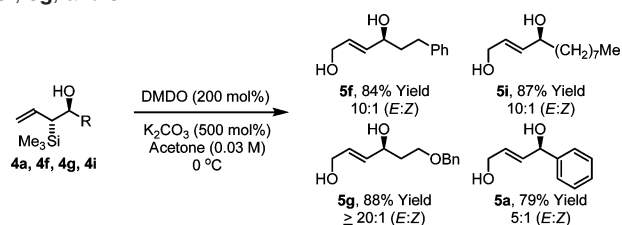
Scheme 3. Dioxirane-Mediated Oxidative Desilylation of Adducts 4a , 4f , 4g , and 4i to Furnish the Corresponding 1,4-Ene-diols 5a , 5f , 5g , and 5i
