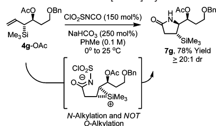
Scheme 5. Reaction of Adduct 4g with Chlorosulfonyl Isocyanate to Furnish the Product of Formal [3 + 2] Cycloaddition 7g
