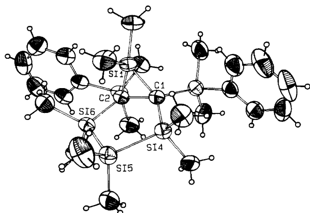
Fig. 3. ORTEP drawing of 30 . Selected bond lengths (Å) and angles (°): Si(1)–C(1) 1.832(4); Si(1)–C(2), 1.843(4); C(1)–C(2), 1.686(5); C(1)–Si(4), 1.916(4); C(2)–Si(6), 1.920(4); Si(4)–Si(5), 2.337(2); Si(5)–Si(6), 2.331(2); C(1)–Si(1)–C(2), 54.6(2); C(1)–C(2)–Si(1), 62.4(2); C(2)–C(1)–Si(1), 63.0(2); Si(1)–C(1)–Si(4), 116.9(2); Si(1)–C(2)–Si(6), 111.9(2); C(1)–Si(4)–Si(5), 105.9(1); Si(4)–Si(5)–Si(6), 94.59(6); C(2)–Si(6)–Si(5), 104.6(1).
