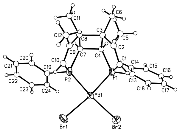
Figure 5. Perspective drawing of \{(DMPP)_2[2 + 2]\}PdBr_2 showing the atom numbering scheme (50% probability ellipsoids). Hydrogen atoms have an arbitrary radius of 0.1 Å.
