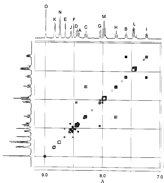
Fig. 5 400 MHz ^1\text{H} 2D-EXSY NMR spectrum of [\text{Pt}(\text{C}_6\text{F}_4\text{CF}_3)_2\text{L}^1] in (\text{CDCl}_3)_2 at 393 K. Mixing time was 0.8 s. Signal labelling refers to Table 3.
