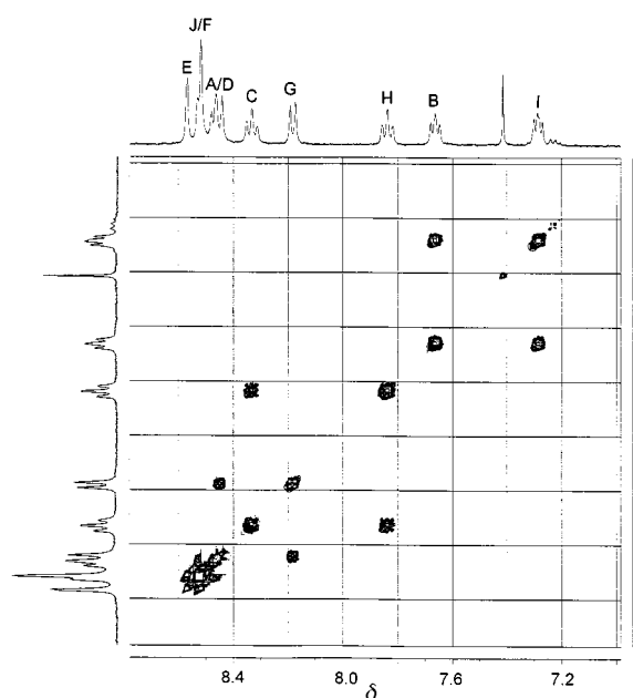
Fig. 4 400 MHz ^1\text{H} 2D-EXSY NMR spectrum of [\text{Pt}(\text{C}_6\text{F}_4\text{CF}_3)_2\text{L}^1] in (\text{CDCl}_2)_2 at 393 K. Mixing time was 0.8 s. Signal labelling refers to Table 2.
