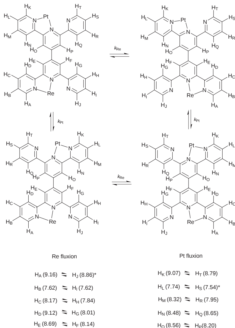
Fig. 2 Interconversion of the four equivalent structures of [\text{ReBr}(\text{CO})_3\text{Pt}(\text{Ime}_3)\text{L}] as a result of the \text{Re}^{\text{I}} and \text{Pt}^{\text{IV}} moiety M–N shifts. The chemical shifts of the exchanging pairs of signals are measured at 253 K in (\text{CDCl}_2)_2 solvent. The asterisks refer to the pairs of signals used for bandshape analysis.
