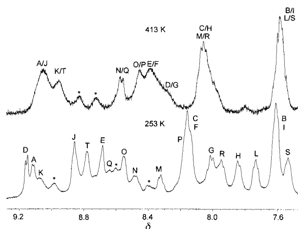
Fig. 3 400 MHz ^1\text{H} spectra of [\text{ReBr}(\text{CO})_3\text{Pt}(\text{Ime}_3)\text{L}] in (\text{CDCl}_2)_2 measured at 253 and 413 K. The asterisks denote impurity bands of [\text{ReBr}(\text{CO})_3\text{L}] . See Fig. 2 for signal labelling.
