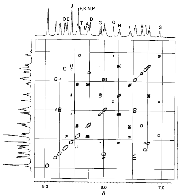
Fig. 8 400 MHz ^1H 2D-COSY45 NMR spectrum of [Pt(C_6F_5)_2L^3] in (CDCl_2)_2 at 353 K. Labelling refers to Table 6 and Fig. 7. The unlabelled signals are due to hydrogens on the un-coordinated side of the ligand.
