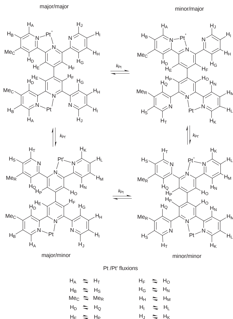
Fig. 7 Interconversion of the four structures of [(Pt(Ime)_3)_2L^3] following Pt^{IV} moiety fluxions.
