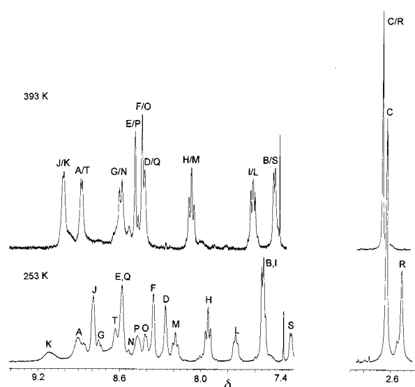
Fig. 6 400 MHz ^1\text{H} NMR spectrum of [(\text{PtIme}_3)_2\text{L}^3] in (\text{CDCl}_2)_2 at 253 and 393 K, the slow and fast exchange limits of Pt–N metallotropic shifts. Signal labelling refers to Table 6.
