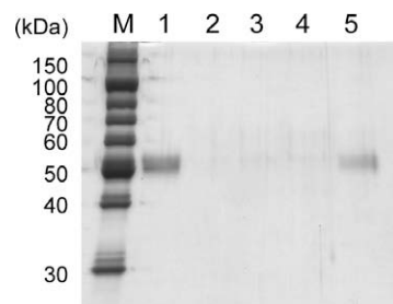
Figure 3. Binding of neuraminidase (rvH1N1NA) to resin-conjugated Tamiflu analog 3 . Binding assay of rvH1N1NA was performed for 3 . The eluted protein was analyzed by SDS-PAGE and was visualized by silver staining. A molecular weight of rvH1N1NA is 48 kDa, and it migrates as a 57 kDa band in SDS-PAGE. The position of rvH1N1NA was marked by the arrowhead. rvH1N1NA (lanes 3 and 5) or buffer (lanes 2 and 4) was applied for control resin (lanes 2 and 3) or 3 (lanes 4 and 5). M, molecular weight marker; lane 1, rvH1N1NA standard (0.5 \mu\text{g} ).
