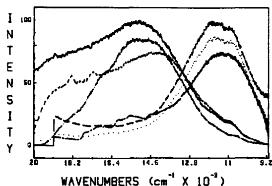
Fig. 4. Corrected luminescence of [(\eta^5\text{-C}_5\text{H}_5)\text{Ru}(\text{DMPP})_2\text{L}]\text{PF}_6 , \text{L} = (\text{CH}_3\text{O})_3\text{P} (—), \text{PhNC} (---), \text{CO} (···), \text{DMPP} (- · - ·), \text{Br} (— — —), and \text{Ph}_3\text{P} (- - -). These spectra were obtained from solid microcrystalline samples at 77 K using 27400\text{ cm}^{-1} ( 365\text{ nm} ) broad band near UV excitation from a mercury/xenon arc lamp. The luminescence band maxima of these complexes occur at 15000 , 14800 , 14200 , 11809 , 11700 and 11400\text{ cm}^{-1} respectively.
