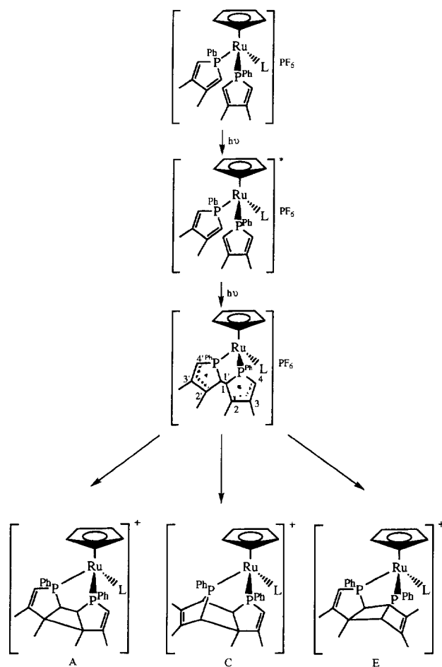
Scheme 3. Proposed mechanism for photochemically induced cycloadditions of [(\eta^5\text{-C}_5\text{H}_5)\text{Ru}(\text{DMPP})_2\text{L}]\text{PF}_6 complexes.
