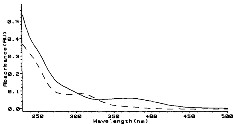
Fig. 3. Electronic absorption spectra of [(\eta^5\text{-C}_5\text{H}_5)\text{Ru}(\text{DMPP})_2\text{L}]\text{PF}_6 in \text{CH}_3\text{CN} , 0.1 cm path length, L = \text{CO} (---) ( 1.48 \times 10^{-4} M), bottom L = \text{CH}_3\text{CN} (—) ( 1.67 \times 10^{-4} M).
